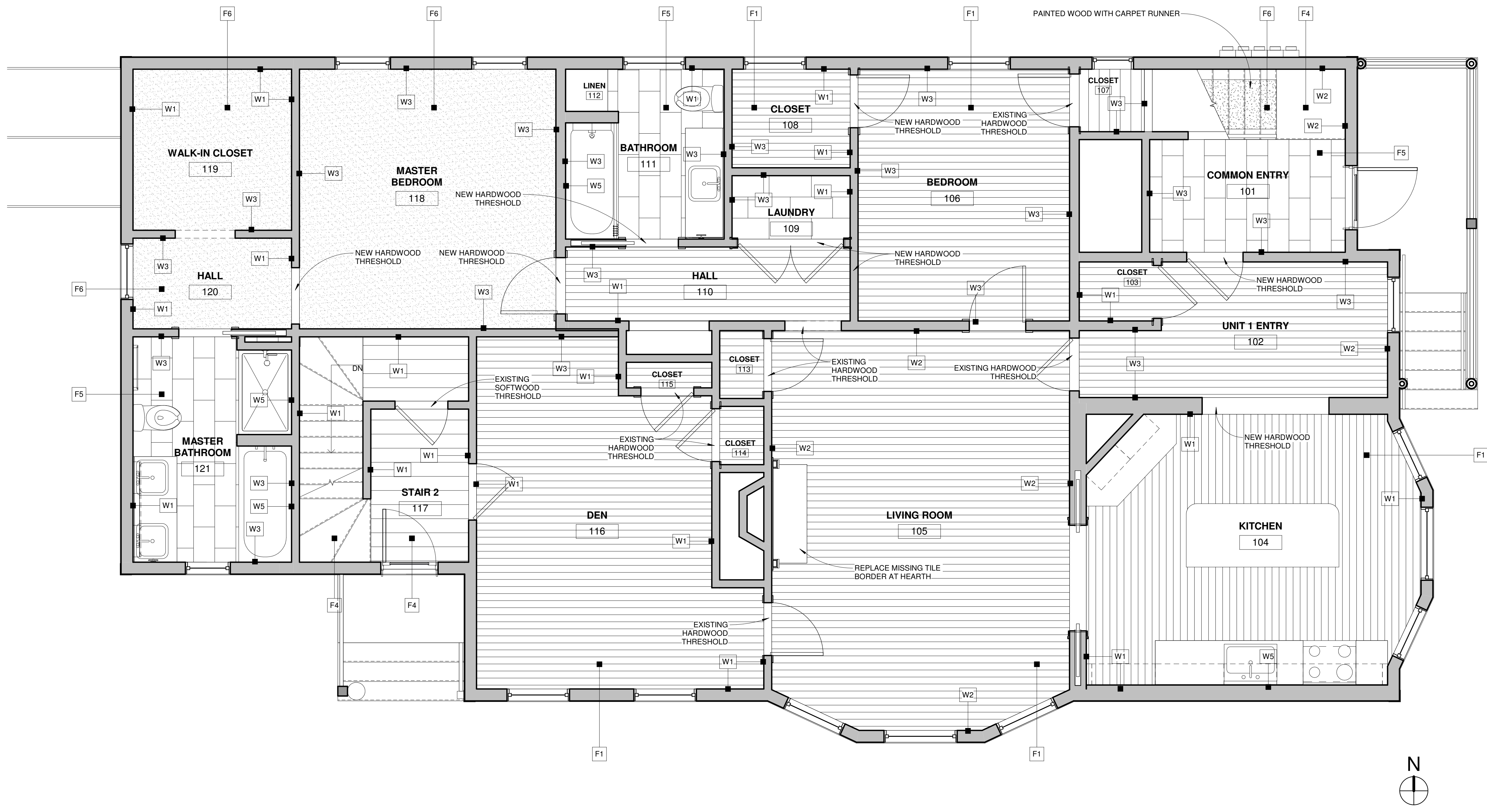
1 UNIT 1 - FINISH PLAN 3/8" = 1'-0"
