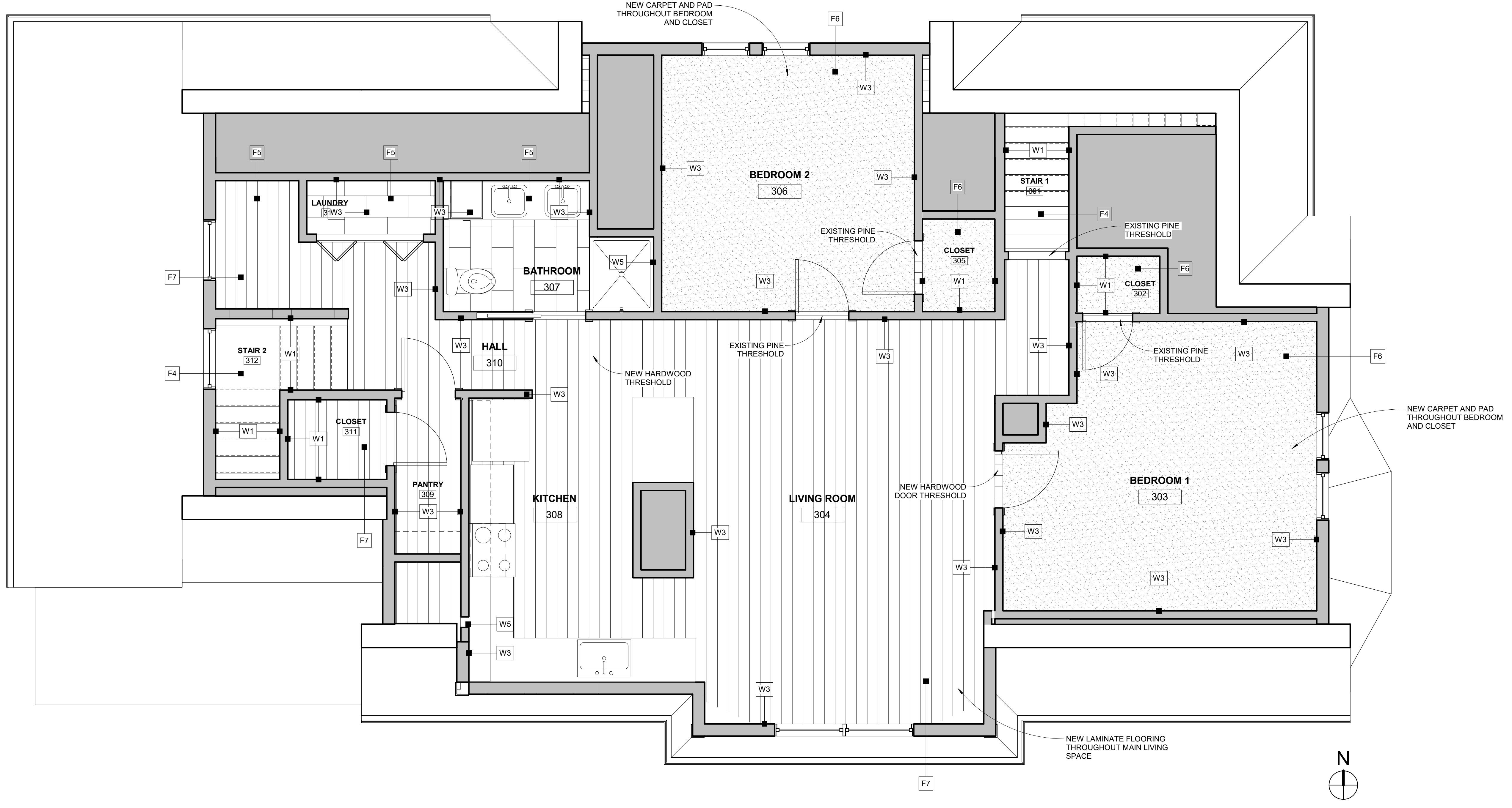
① UNIT 3 - FINISH PLAN 3/8" = 1'-0"
