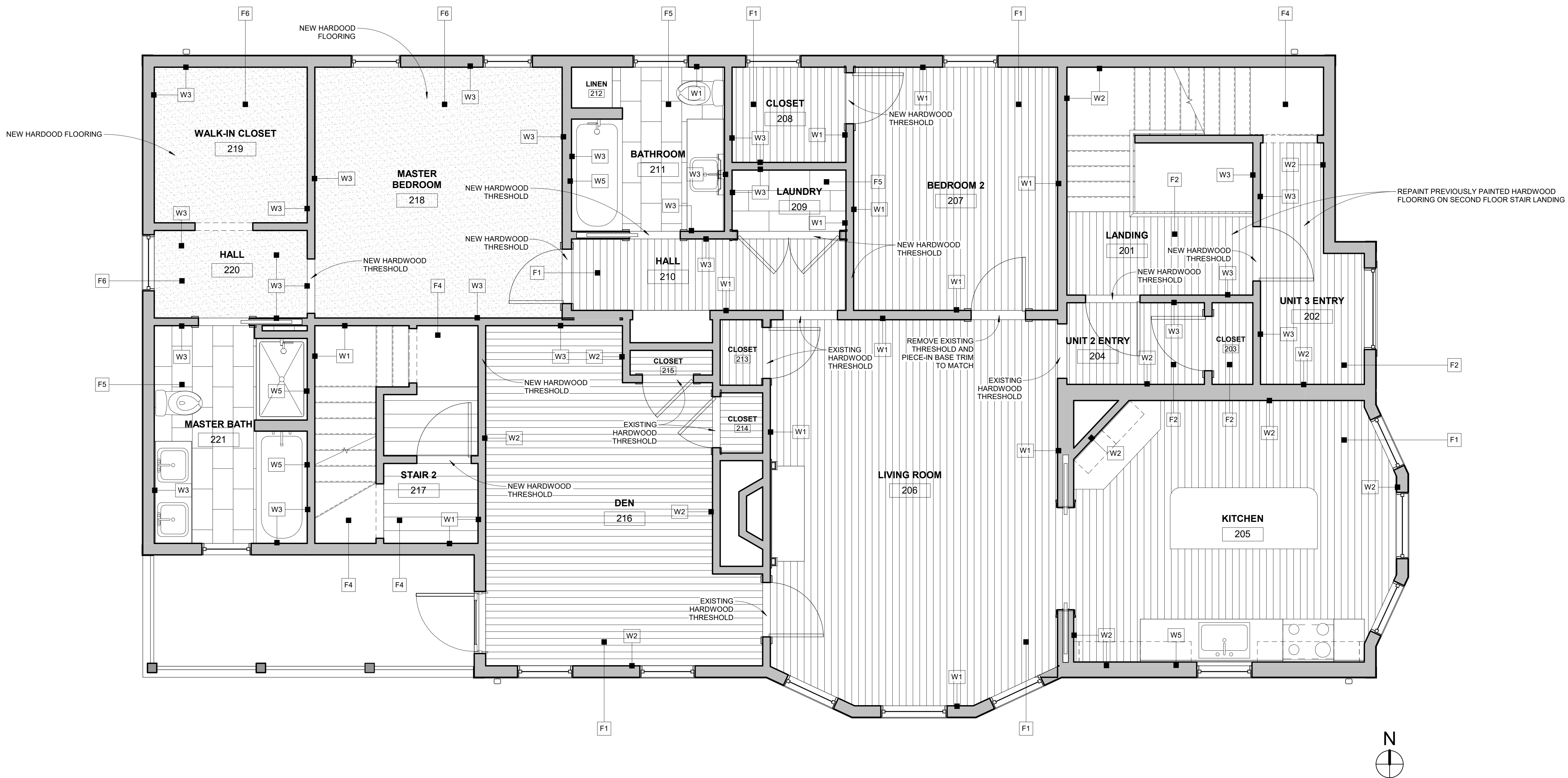
1 UNIT 2 - FINISH PLAN 3/8" = 1'-0"
