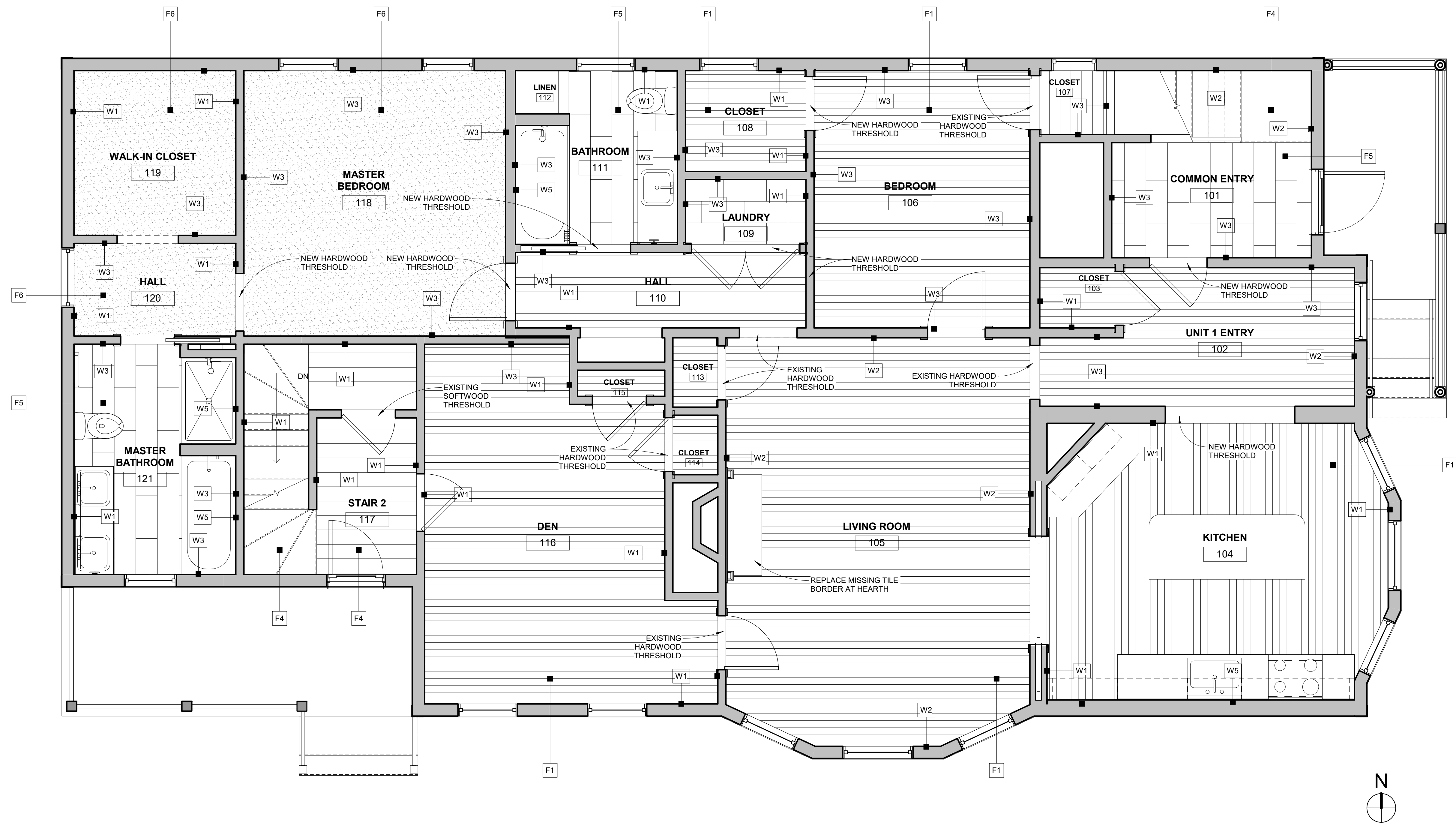
1 UNIT 1 - FINISH PLAN 3/8" = 1'-0"
