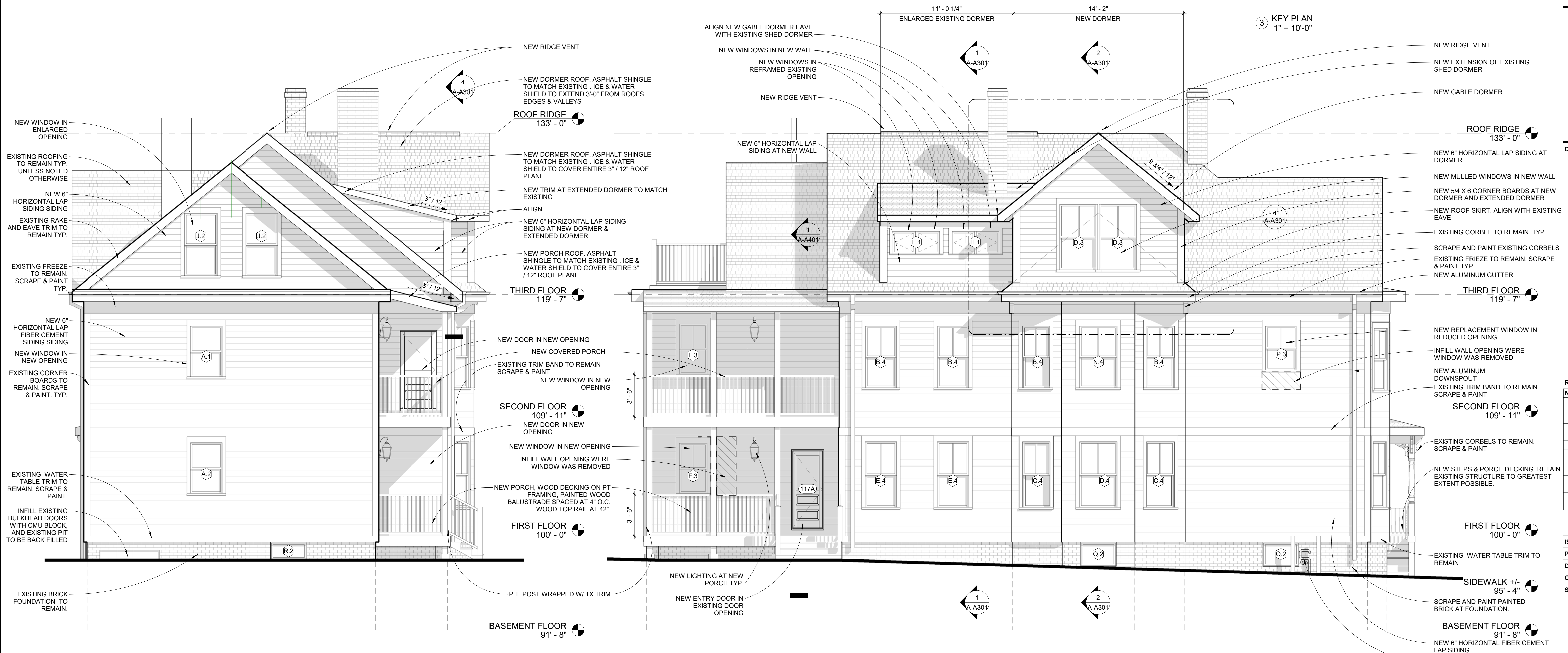
2 EXTERIOR ELEVATION - WEST 1/4" = 1'-0"
