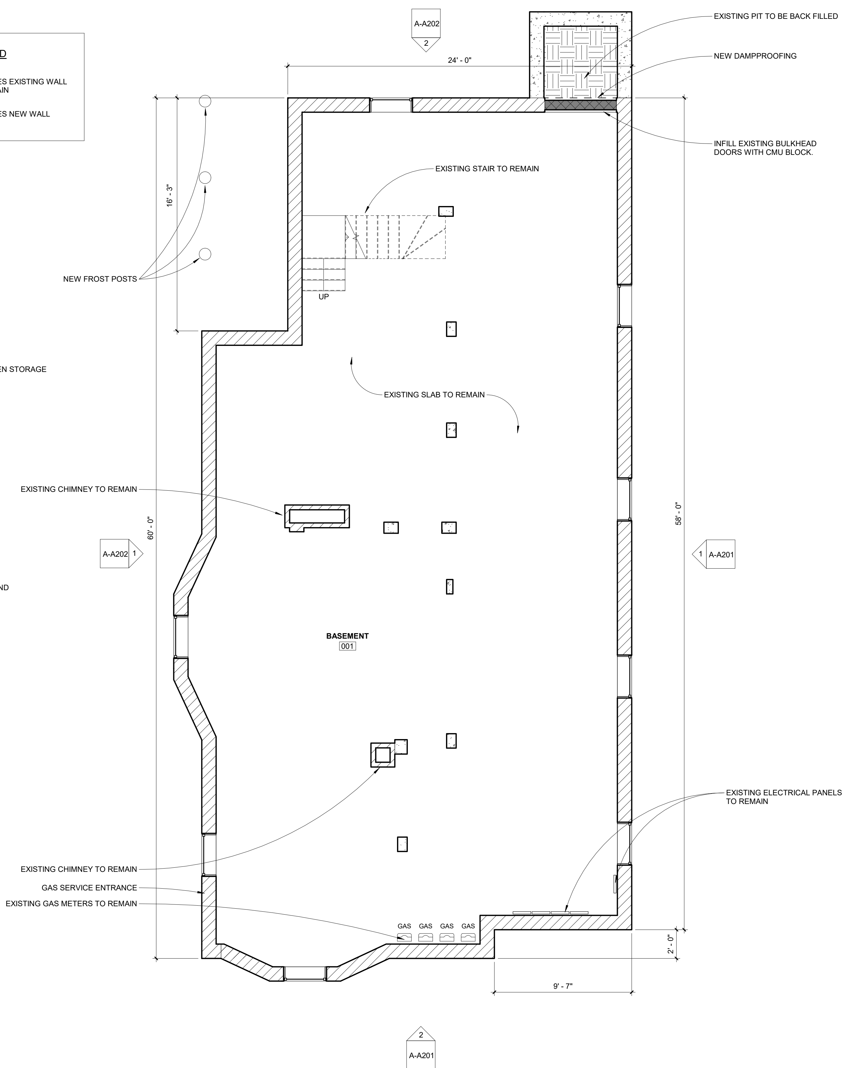
1 BASEMENT PLAN 1/4" = 1'-0"
