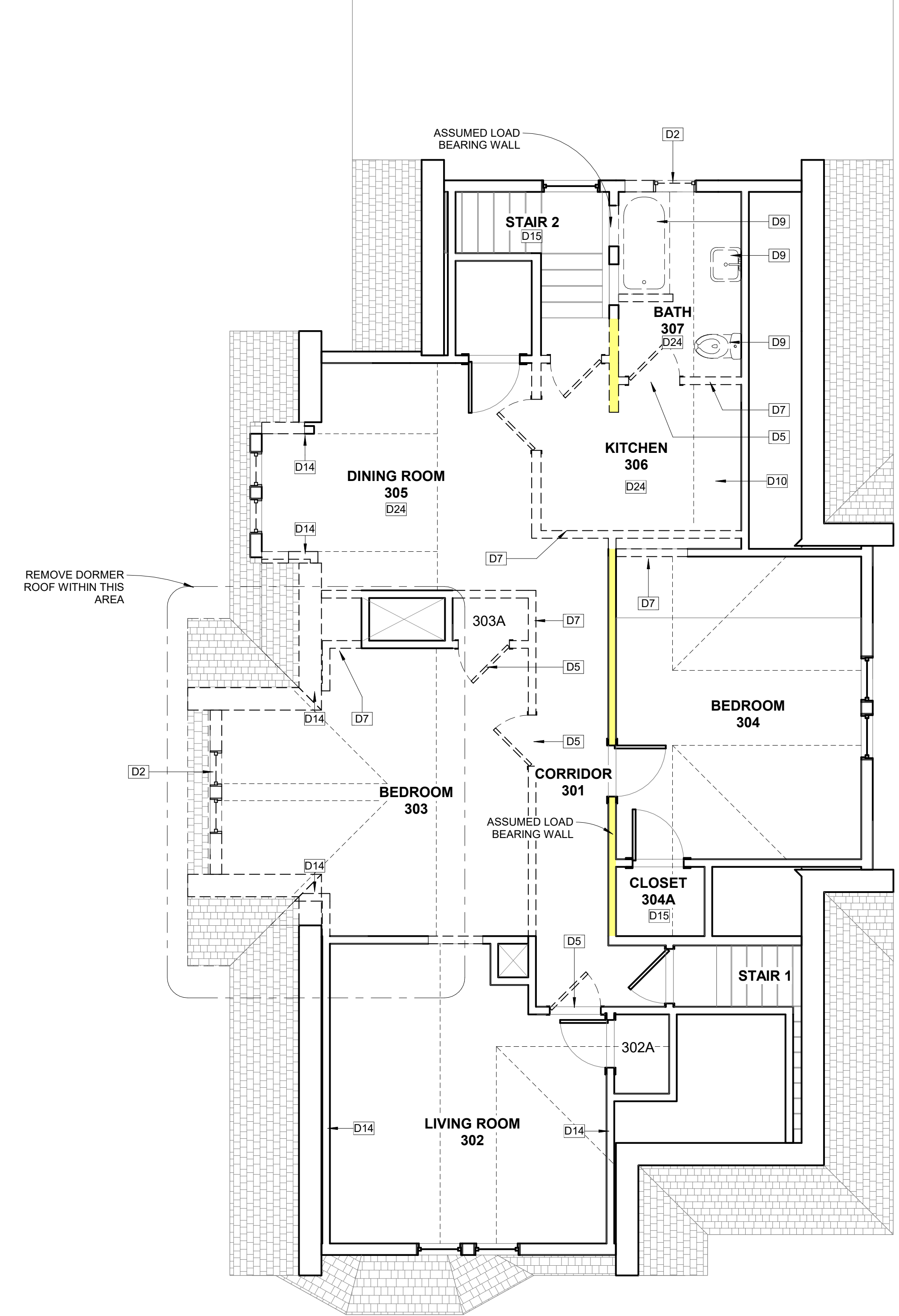
1 THIRD FLOOR DEMO PLAN 1/4" = 1'-0"
