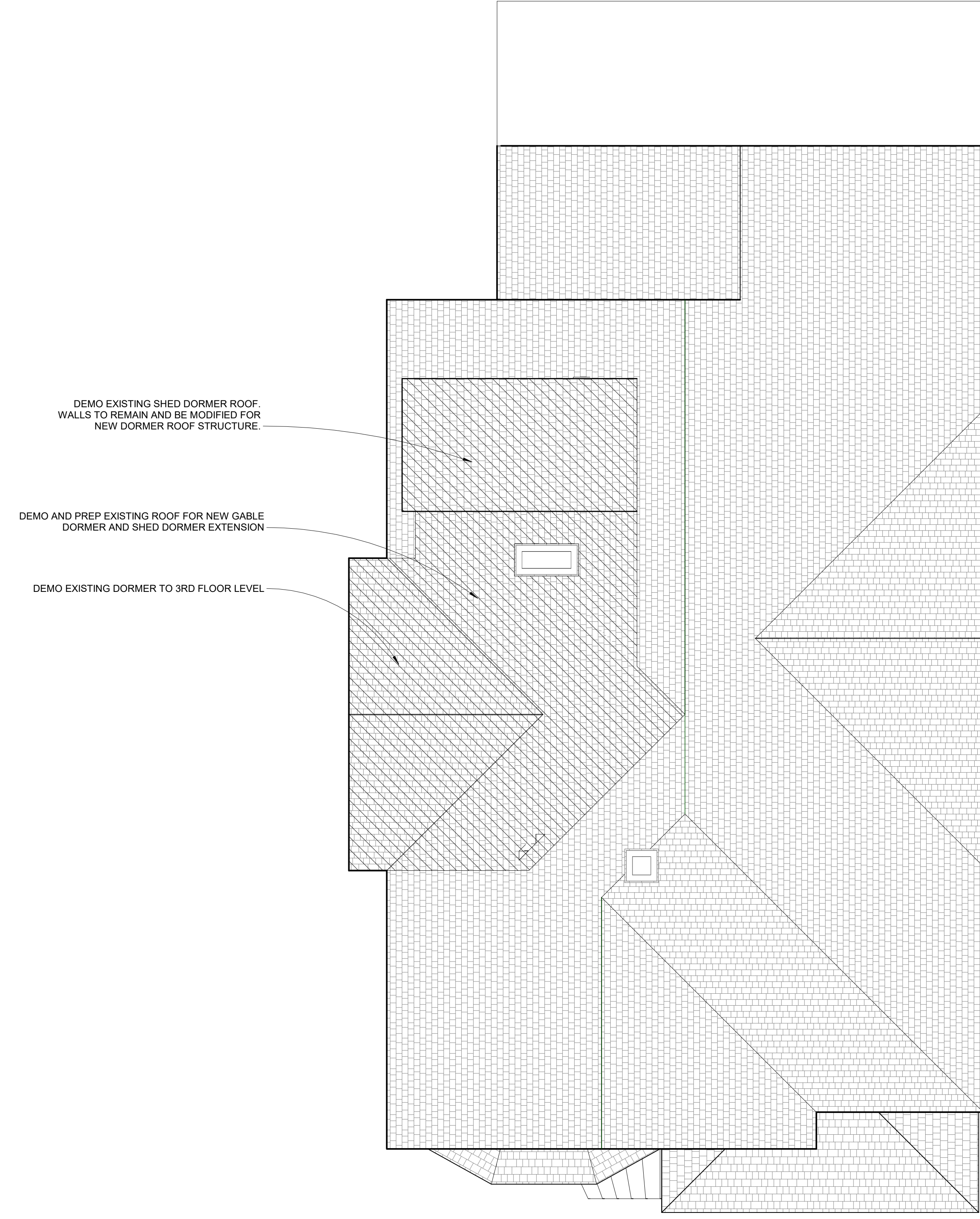
2 DEMO PLAN - Roof 1/4" = 1'-0"
