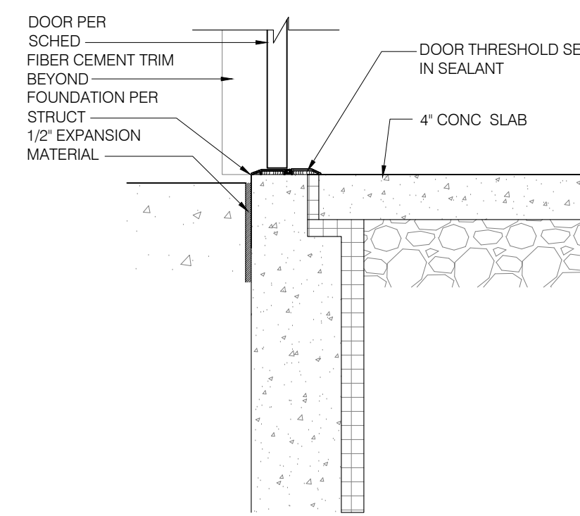
3 THRESHOLD DETAIL SCALE: 1" = 1'-0"
