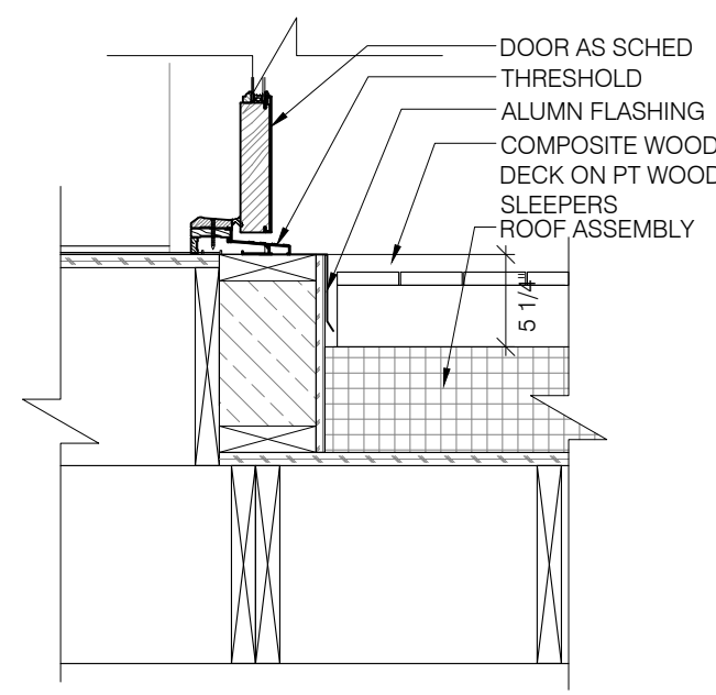
12 ROOF THRESHOLD DETAIL SCALE: 1" = 1'-0"
