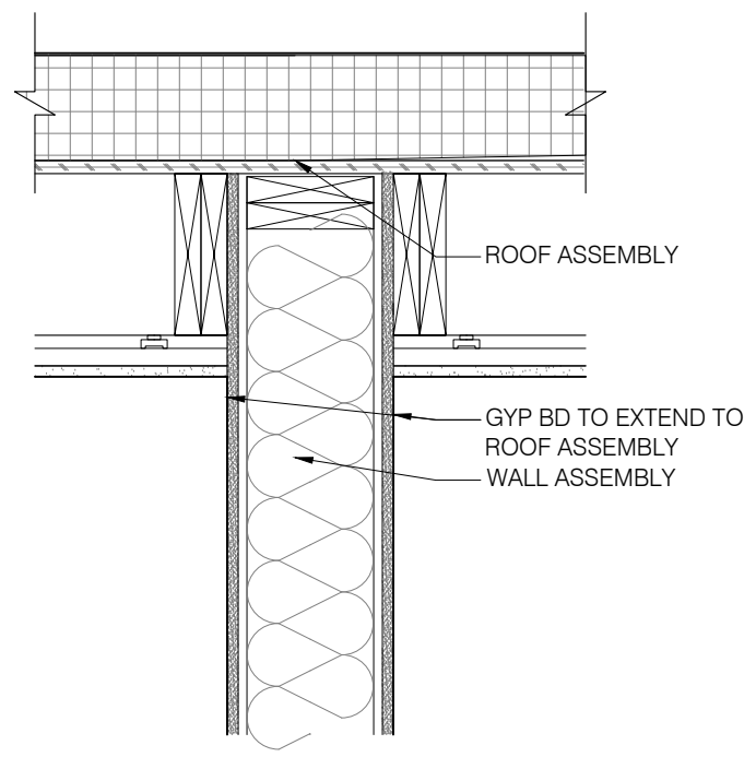
11 RATED WALL DETAIL SCALE: 1" = 1'-0"
