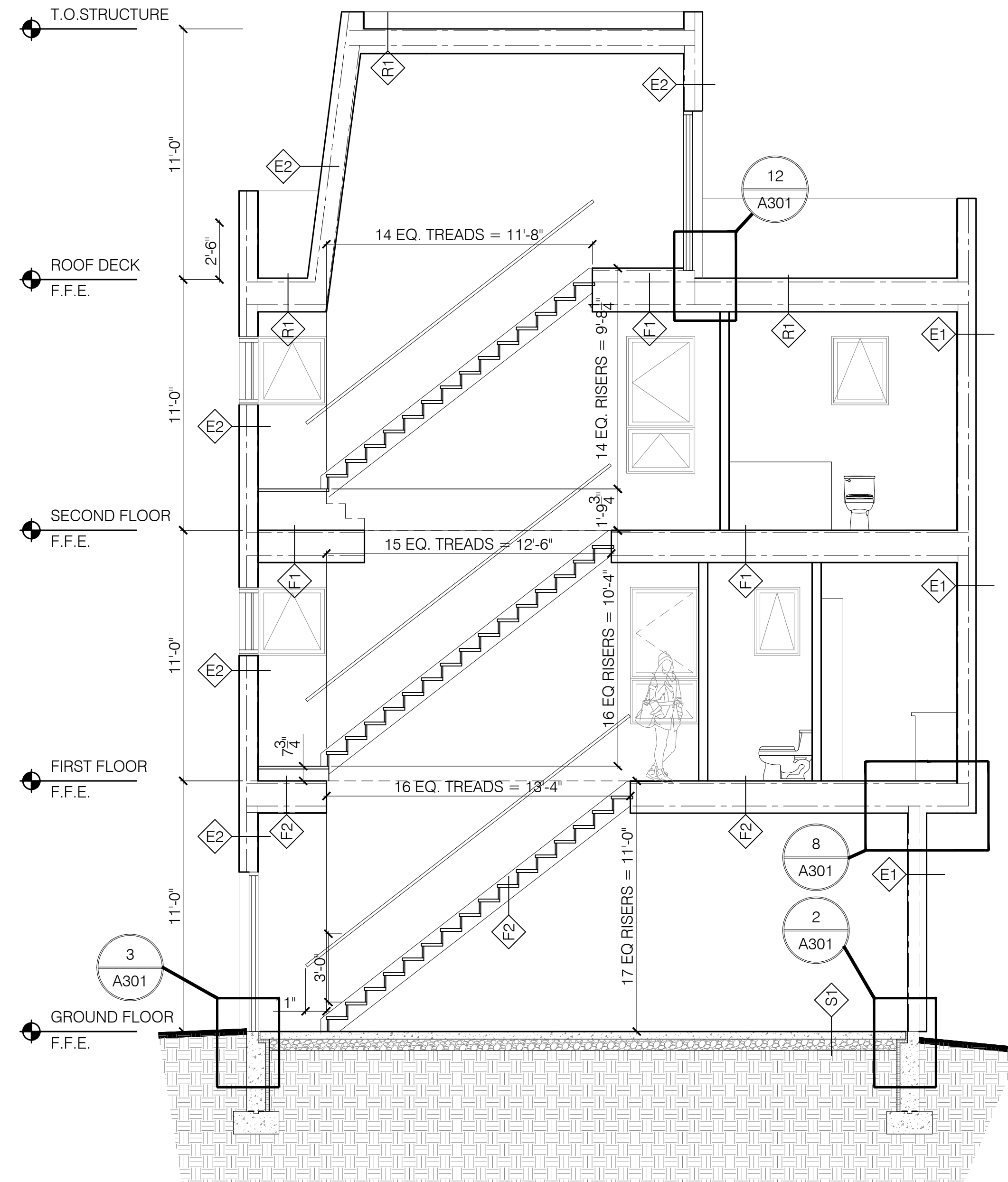
1 BUILDING SECTION SCALE: 1/4" = 1'-0"
