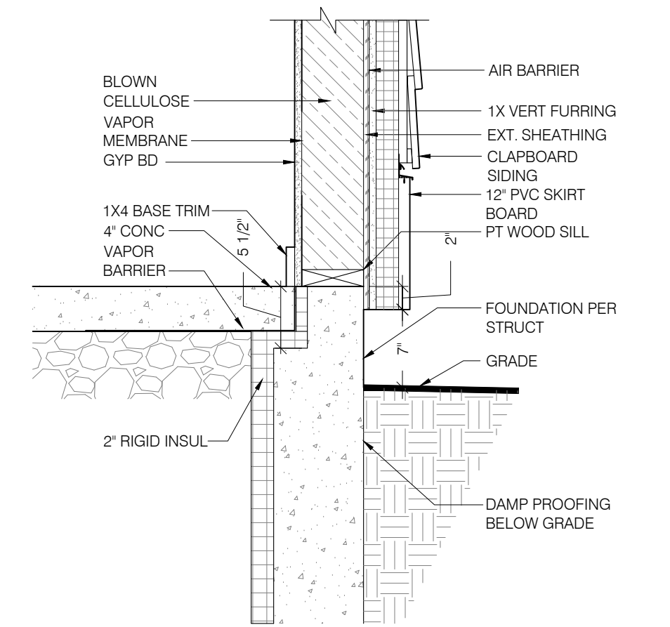
2 FOUNDATION DETAIL SCALE: 1" = 1'-0"
