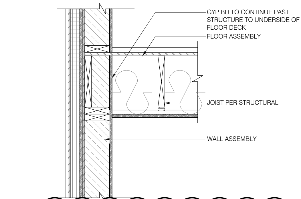
9 EXTERIOR WALL DETAIL SCALE: 1" = 1'-0"
