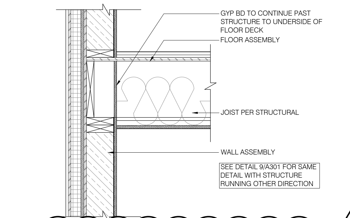
10 EXTERIOR WALL DETAIL SCALE: 1" = 1'-0"
