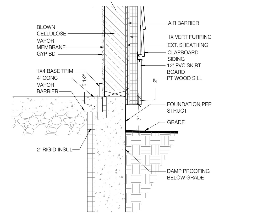
2 FOUNDATION DETAIL SCALE: 1" = 1'-0"
