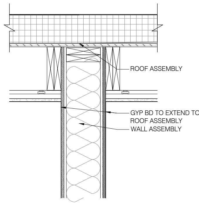
11 RATED WALL DETAIL SCALE: 1" = 1'-0"
