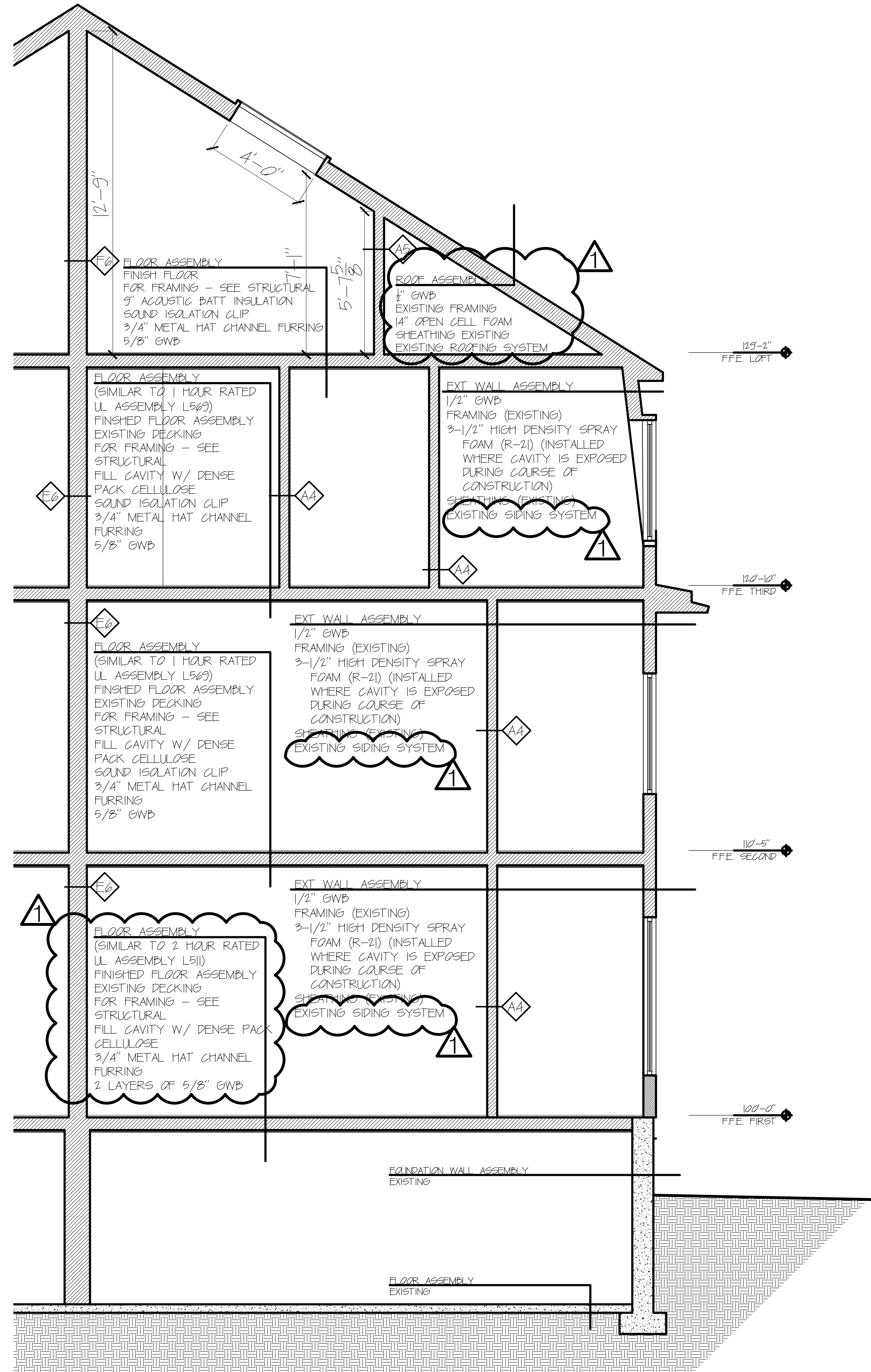
2 TYPICAL BUILDING SECTION SCALE: 3/8" = 1'-0"
