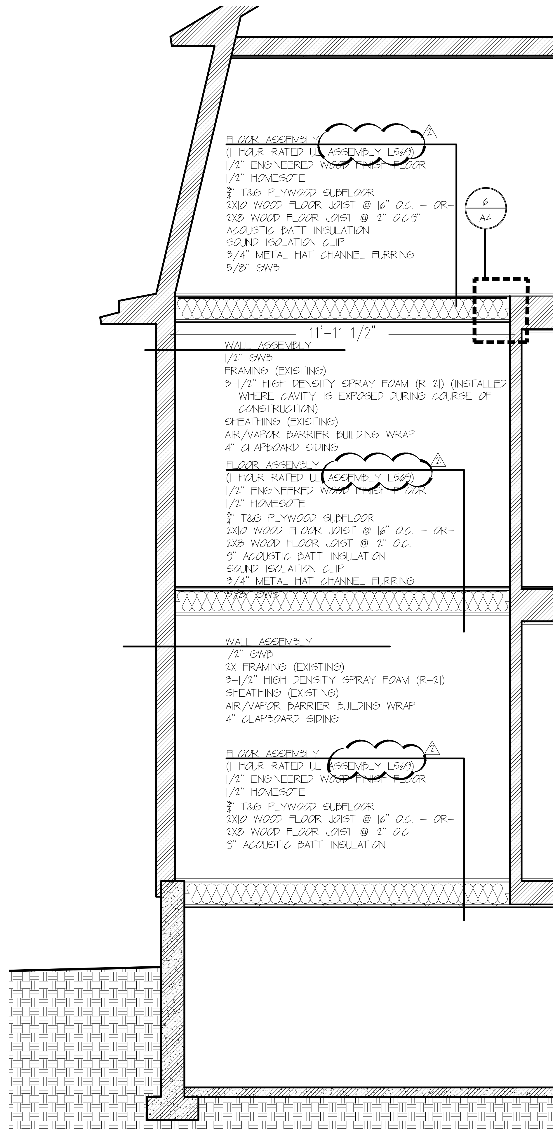
1 STAIR INFILL SECTION 0 2'-0" SCALE: 1/2" = 1'-0"
