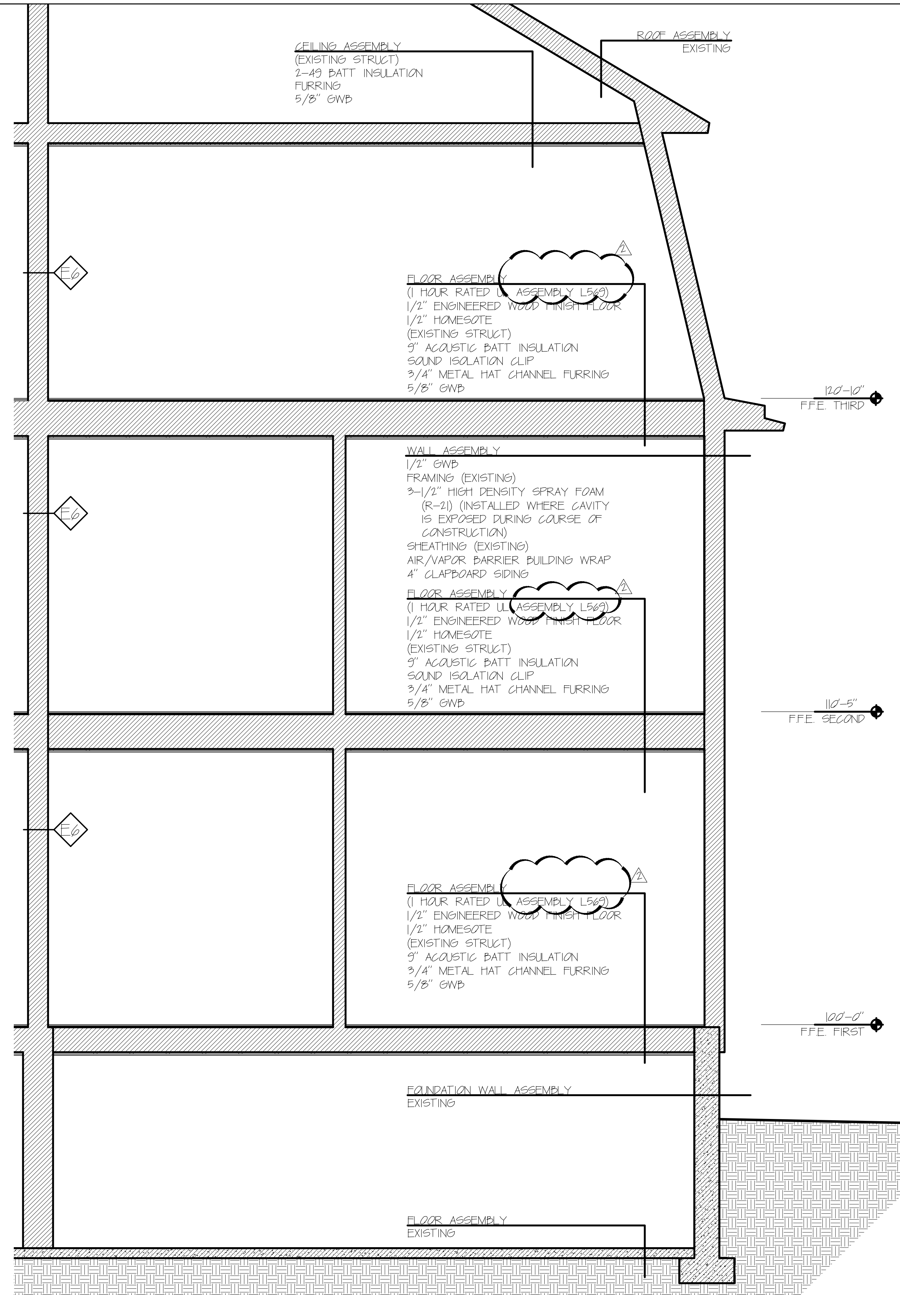
2 TYPICAL BUILDING SECTION 0 2'-0" SCALE: 1/2" = 1'-0"
