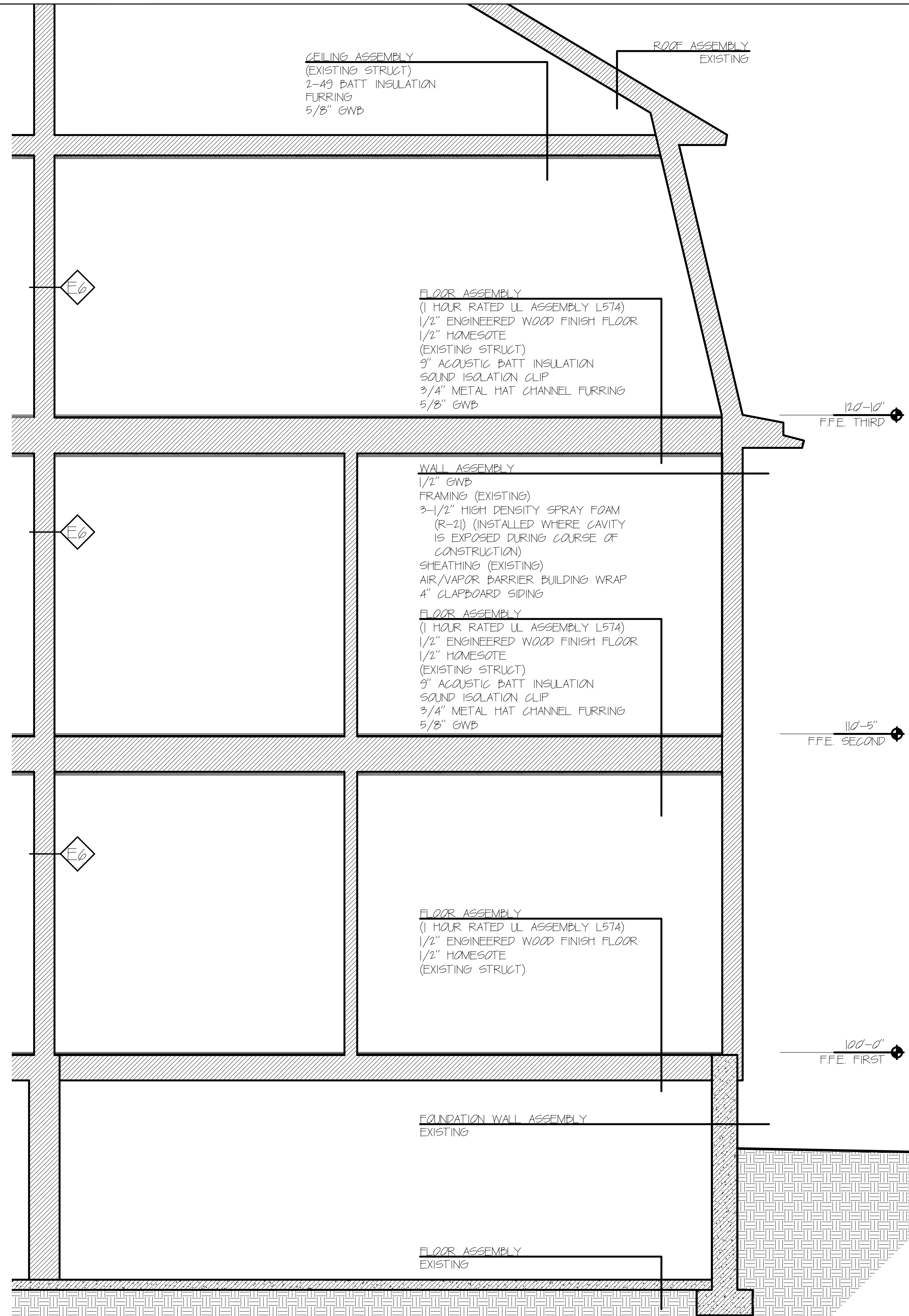
2 TYPICAL BUILDING SECTION 0 2'-0" SCALE: 1/2" = 1'-0"
