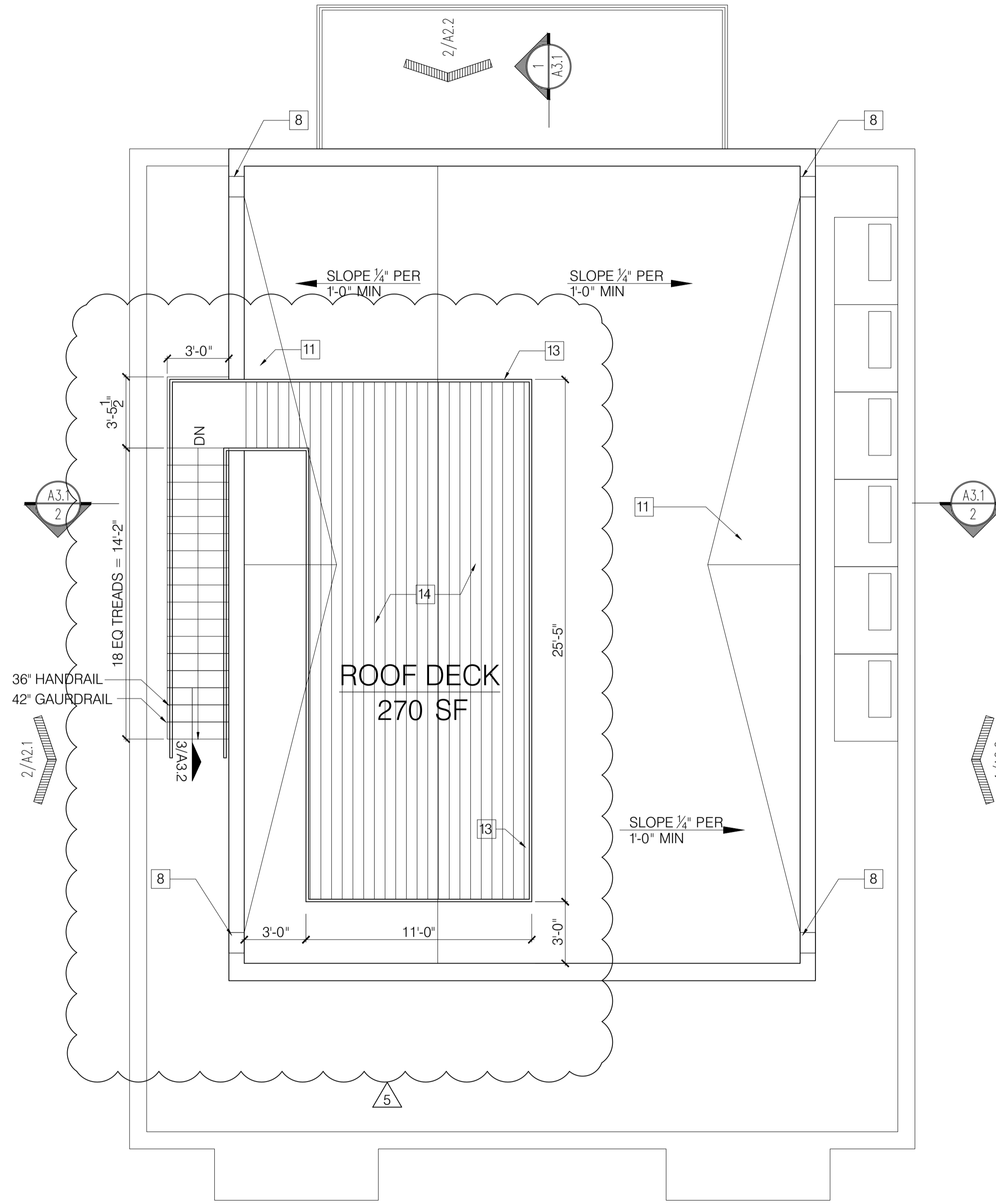
ROOF DECK SCALE: 1/4" = 1'-0"
