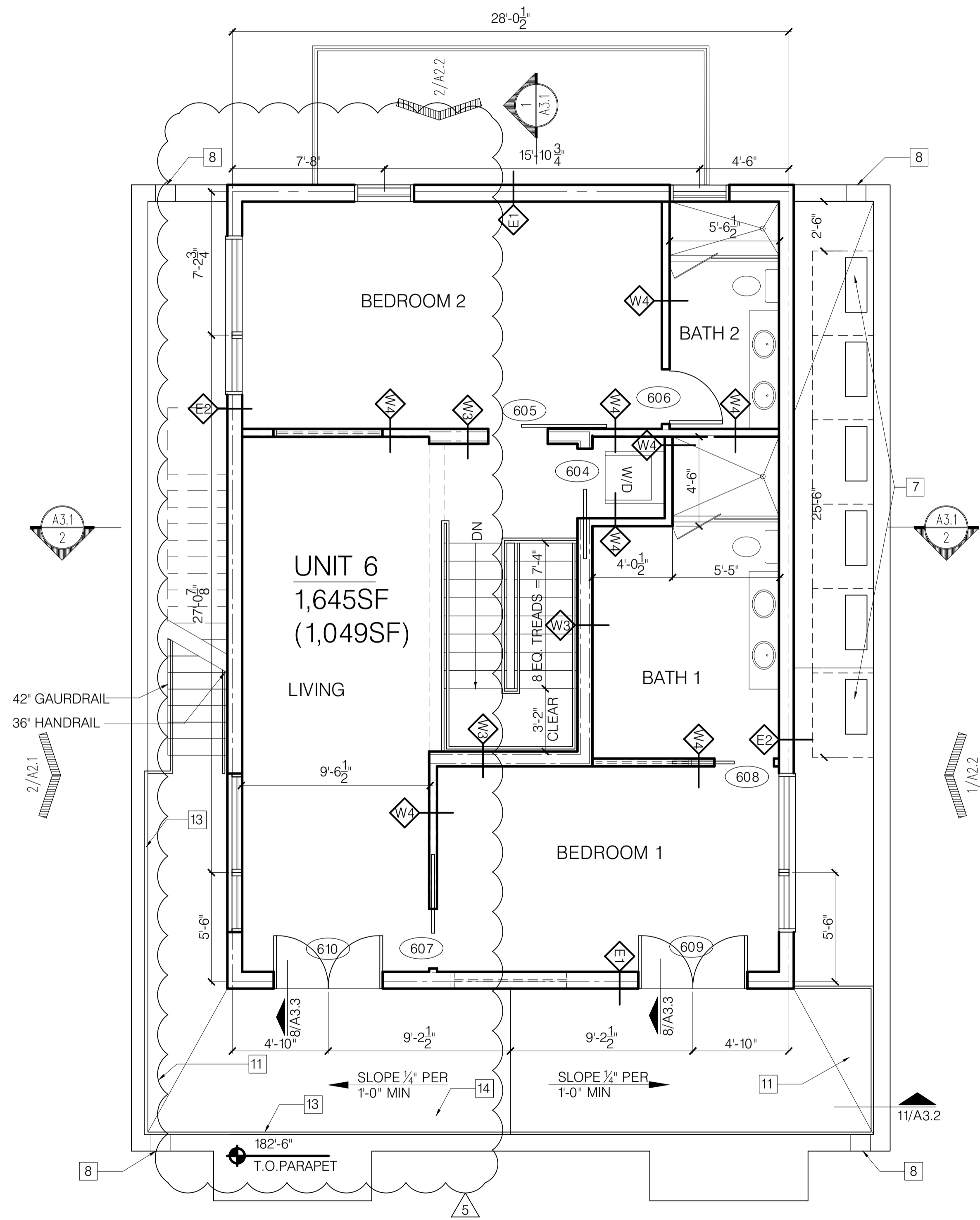
FOURTH FLOOR SCALE: 1/4" = 1'-0"
