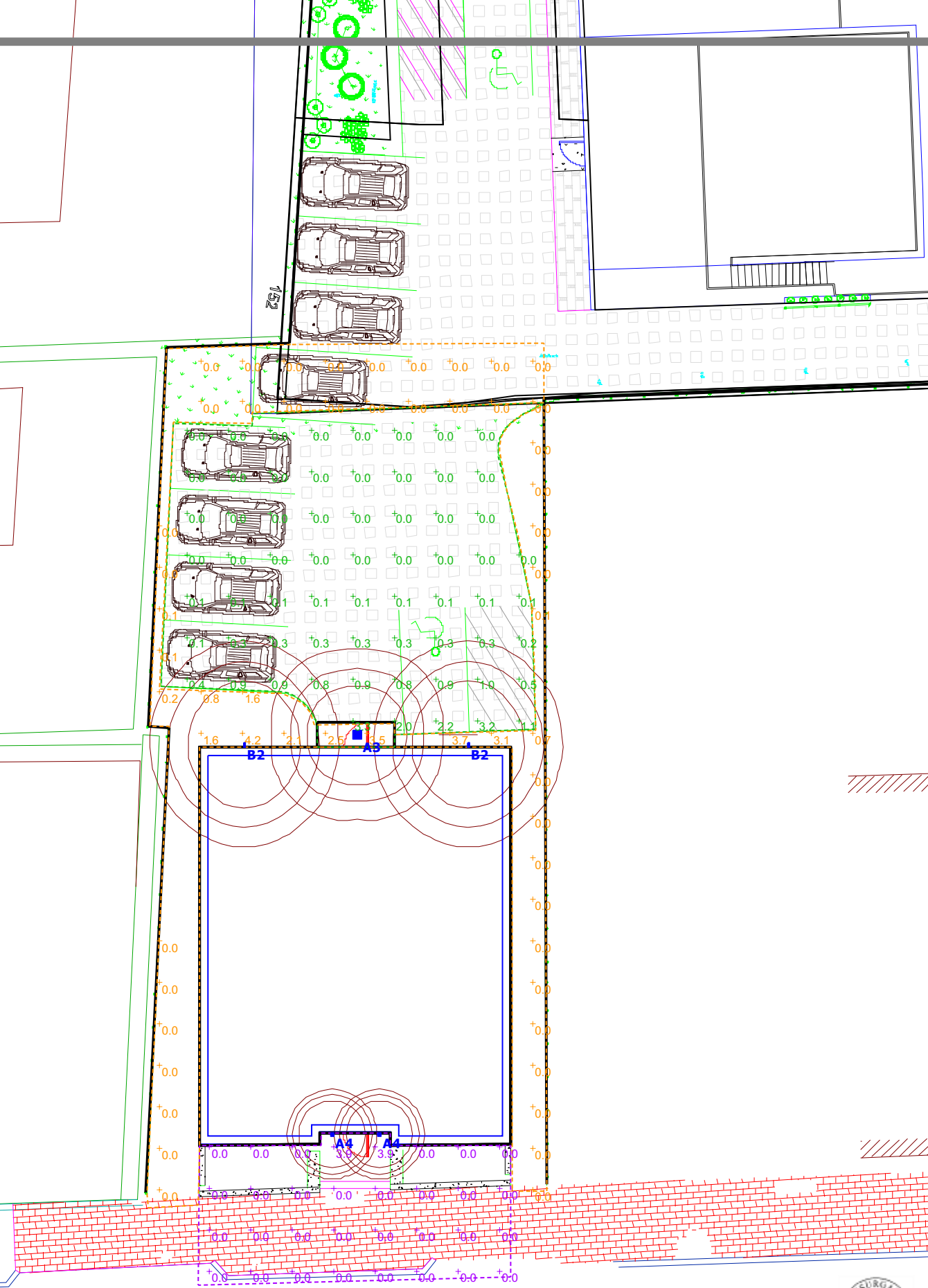
Plan View Scale - 1" = 16ft
