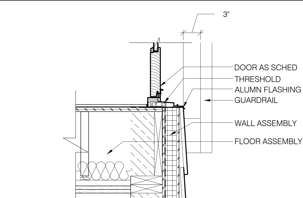
6 SILL - BALCONY DOOR SCALE: 1-1/2" = 1'-0"
