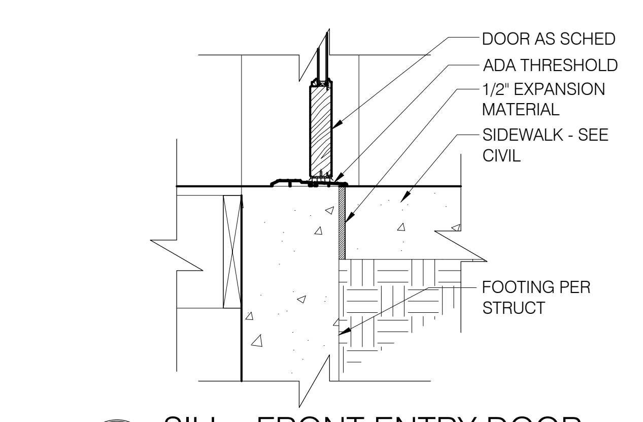
7 SILL - FRONT ENTRY DOOR SCALE: 1-1/2" = 1'-0"
