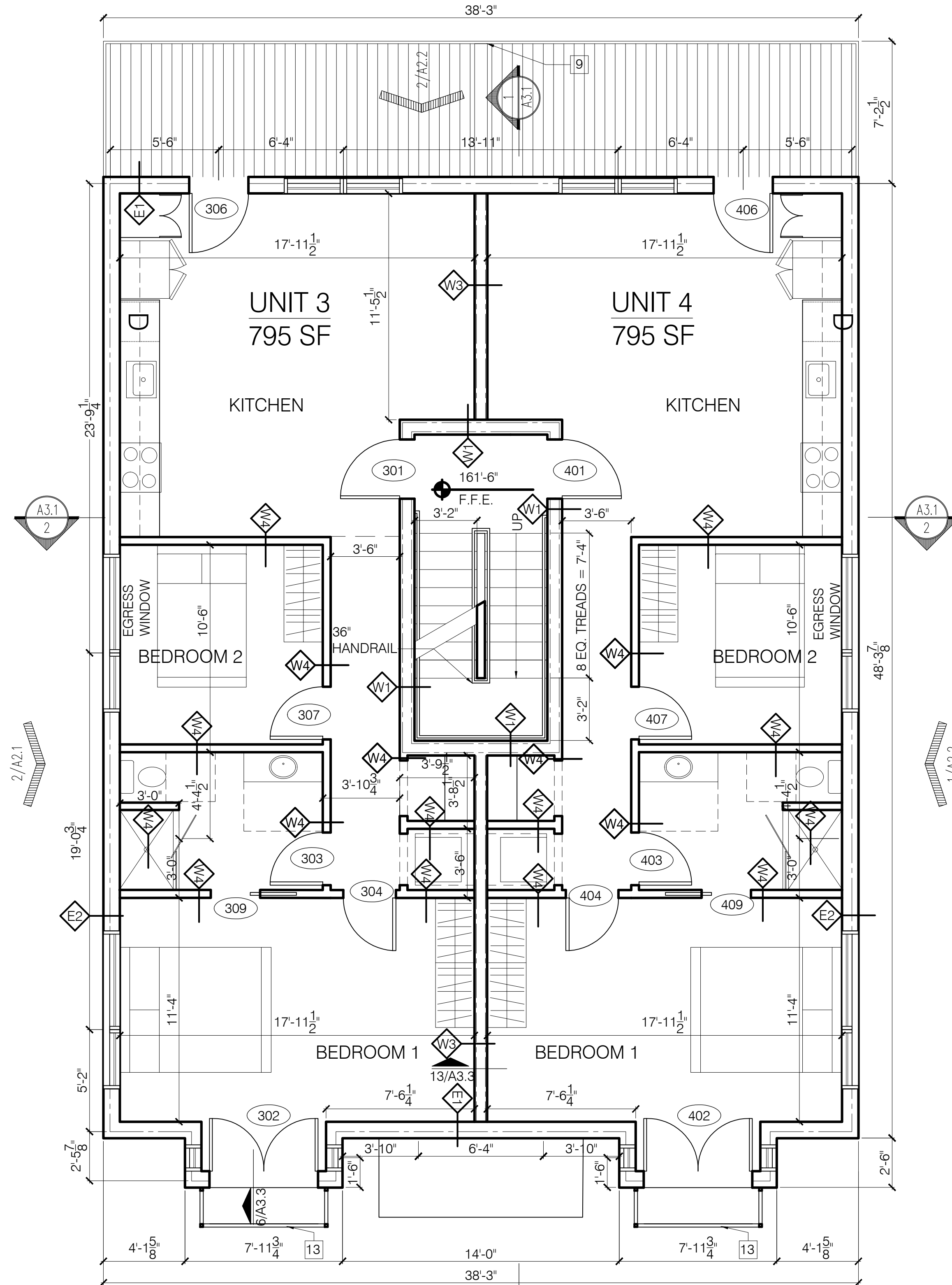
3 SECOND FLOOR SCALE: 1/4" = 1'-0"
