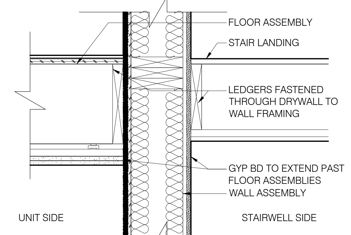
12 RATED WALL STAIR/UNIT SCALE: 1-1/2" = 1'-0"
