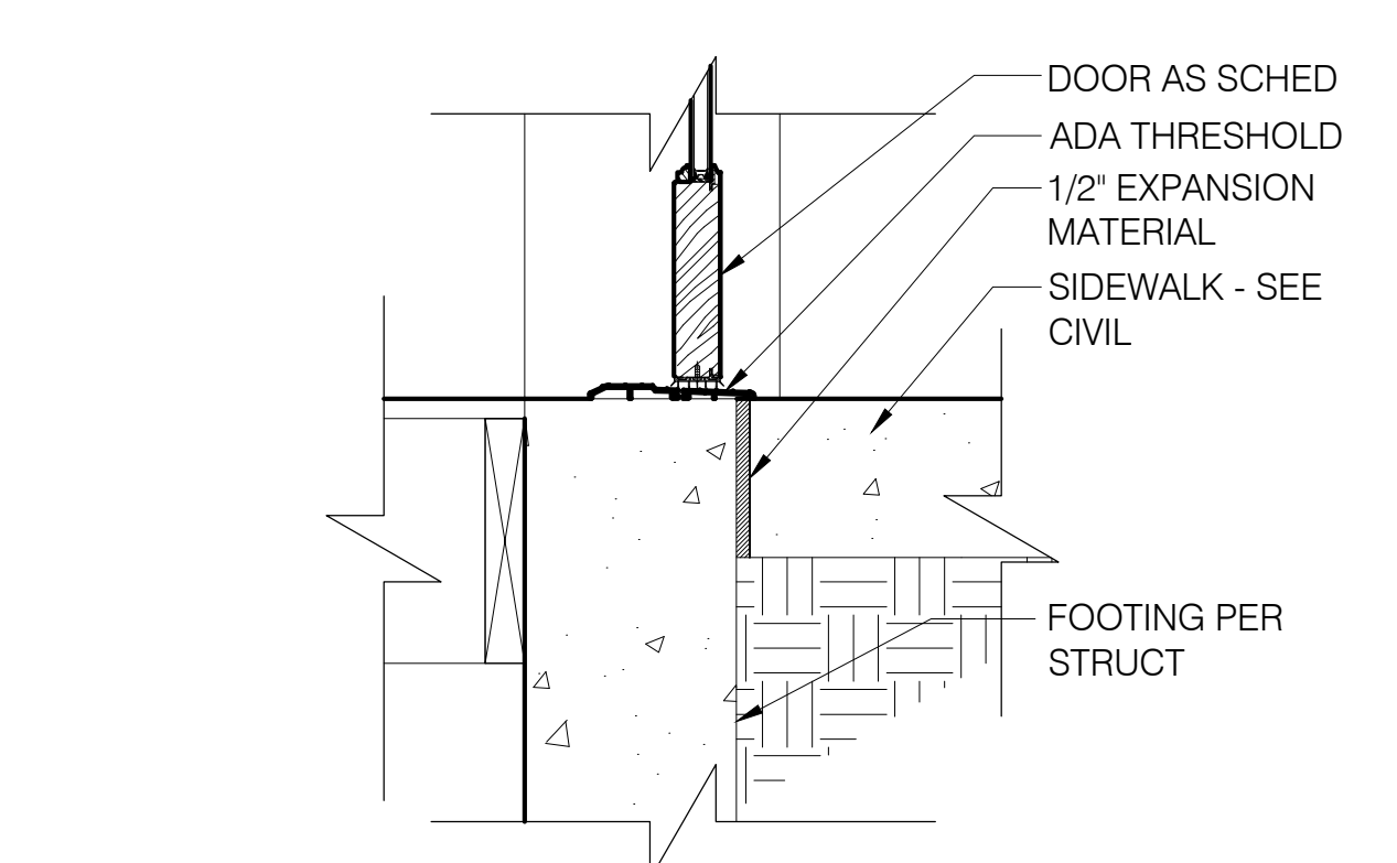
7 SILL - FRONT ENTRY DOOR SCALE: 1-1/2" = 1'-0"
