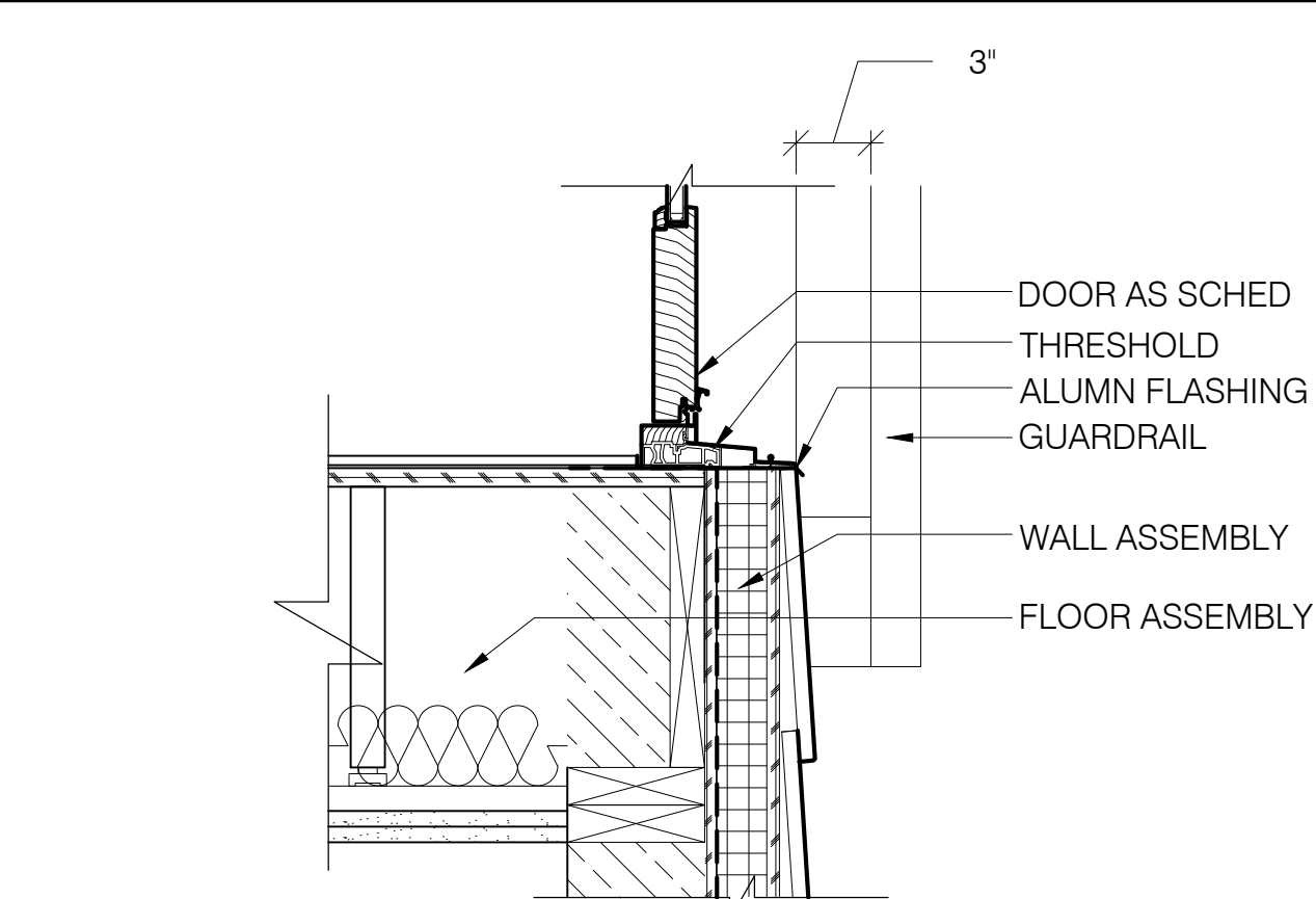
6 SILL - BALCONY DOOR SCALE: 1-1/2" = 1'-0"
