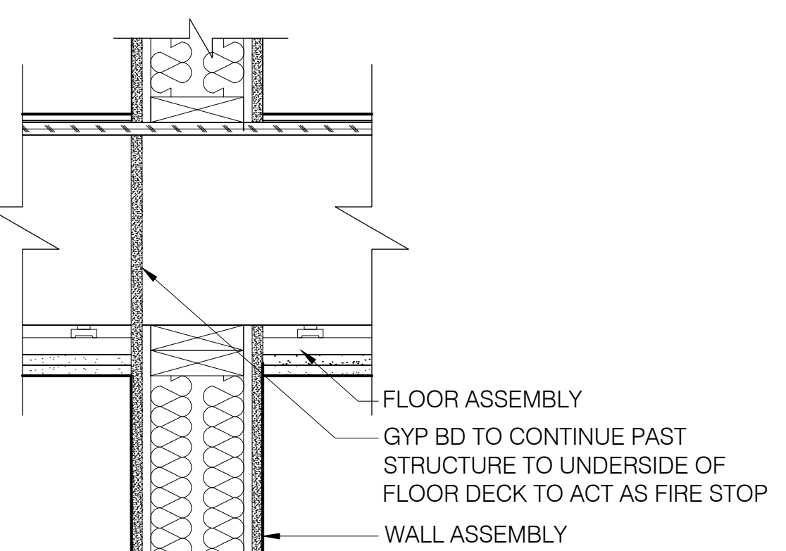
13 RATED WALL BETWEEN UNITS SCALE: 1-1/2" = 1'-0"
