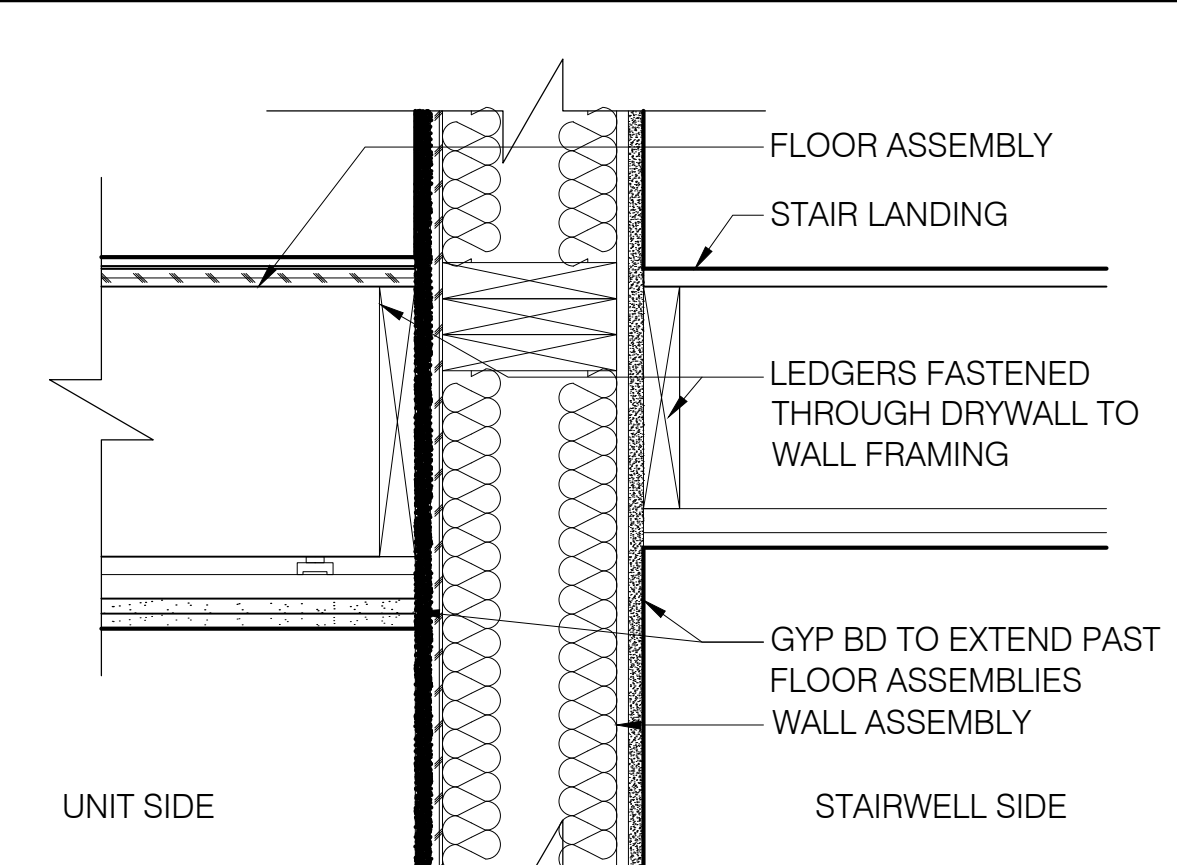
12 RATED WALL STAIR/UNIT SCALE: 1-1/2" = 1'-0"
