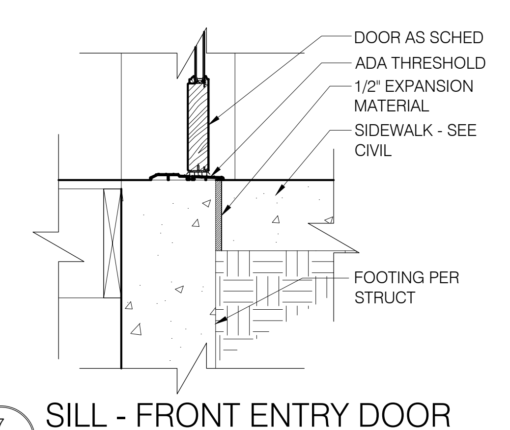
7 SILL - FRONT ENTRY DOOR SCALE: 1-1/2" = 1'-0"
