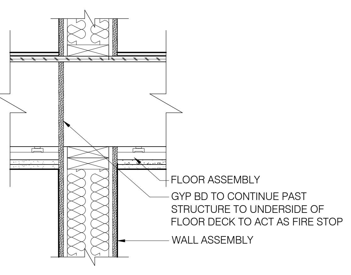
13 RATED WALL BETWEEN UNITS SCALE: 1-1/2" = 1'-0"
