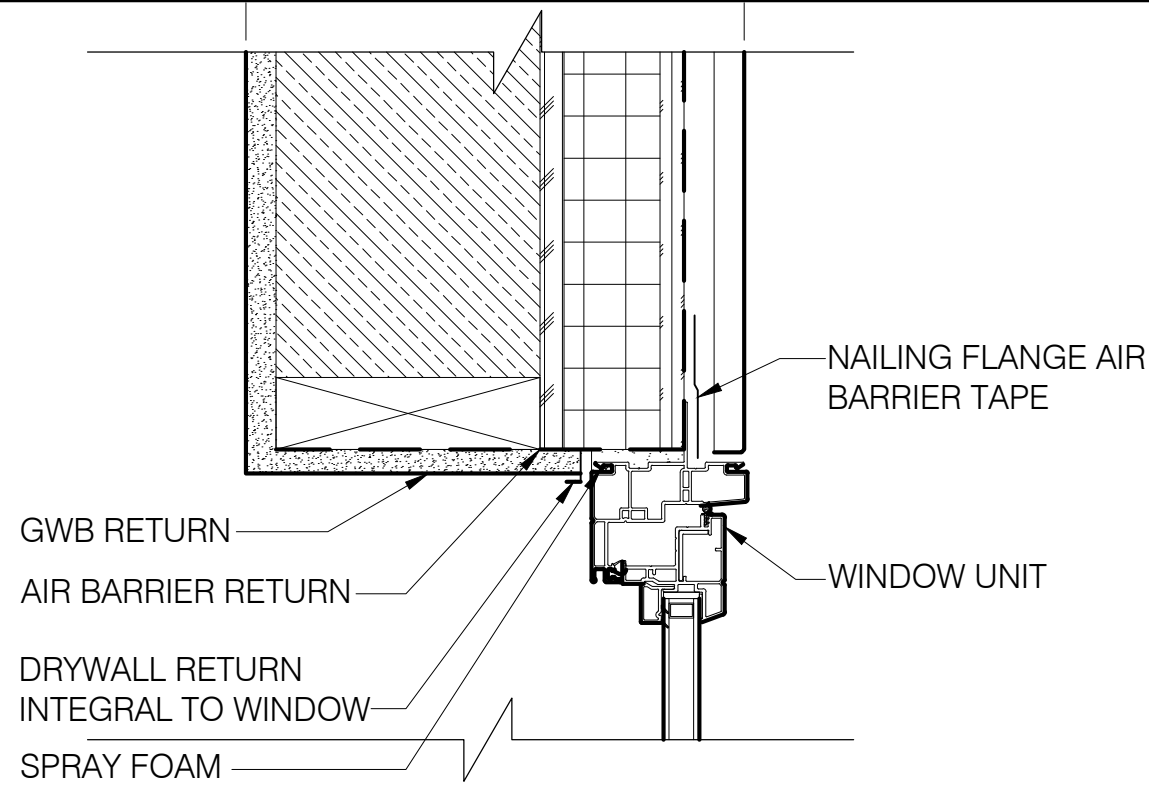
1 HEAD - TYPICAL WINDOW SCALE: 3" = 1'-0"
