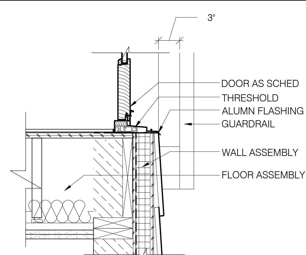
6 SILL - BALCONY DOOR SCALE: 1-1/2" = 1'-0"
