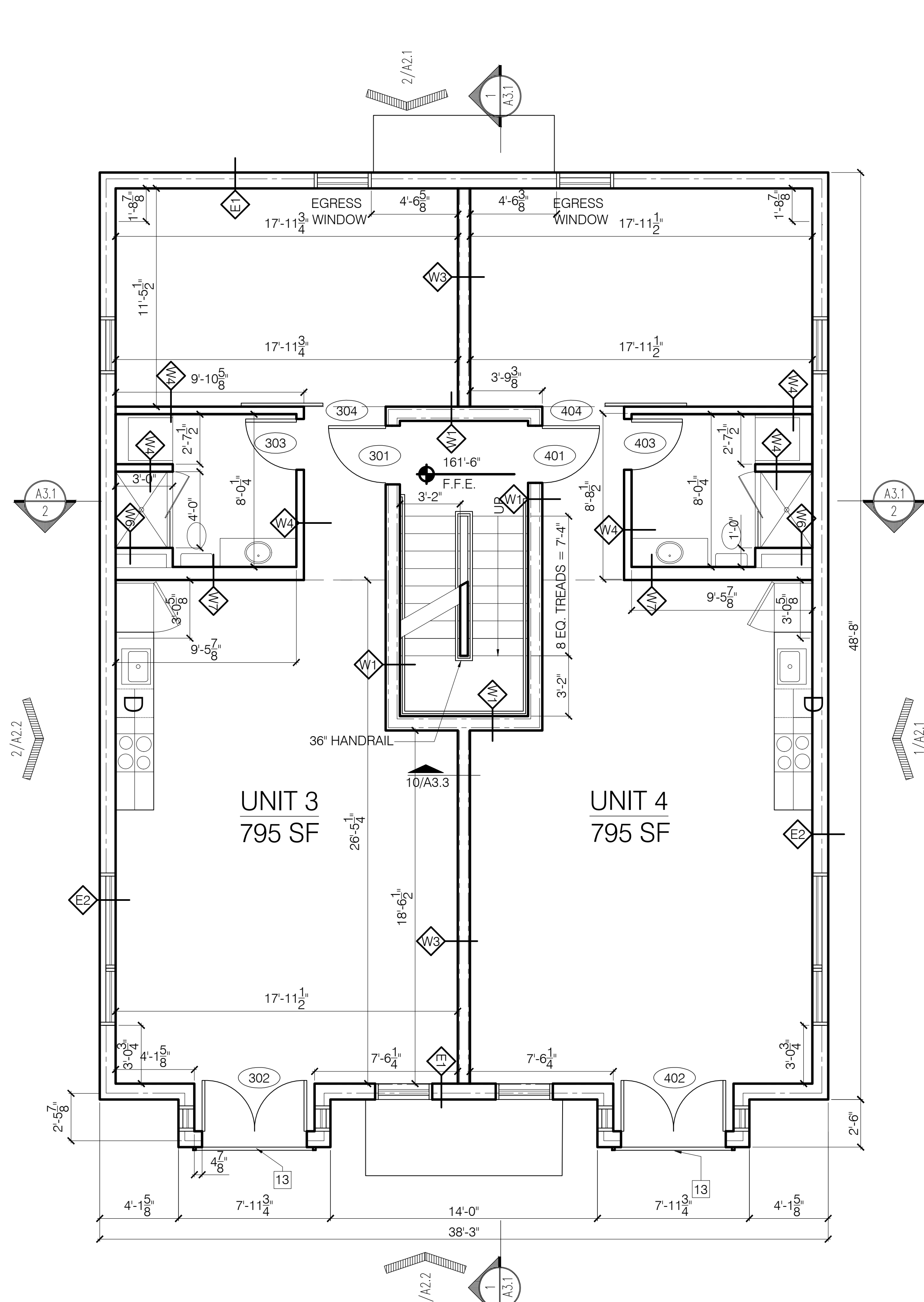
SECOND FLOOR SCALE: 1/4" = 1'-0"
