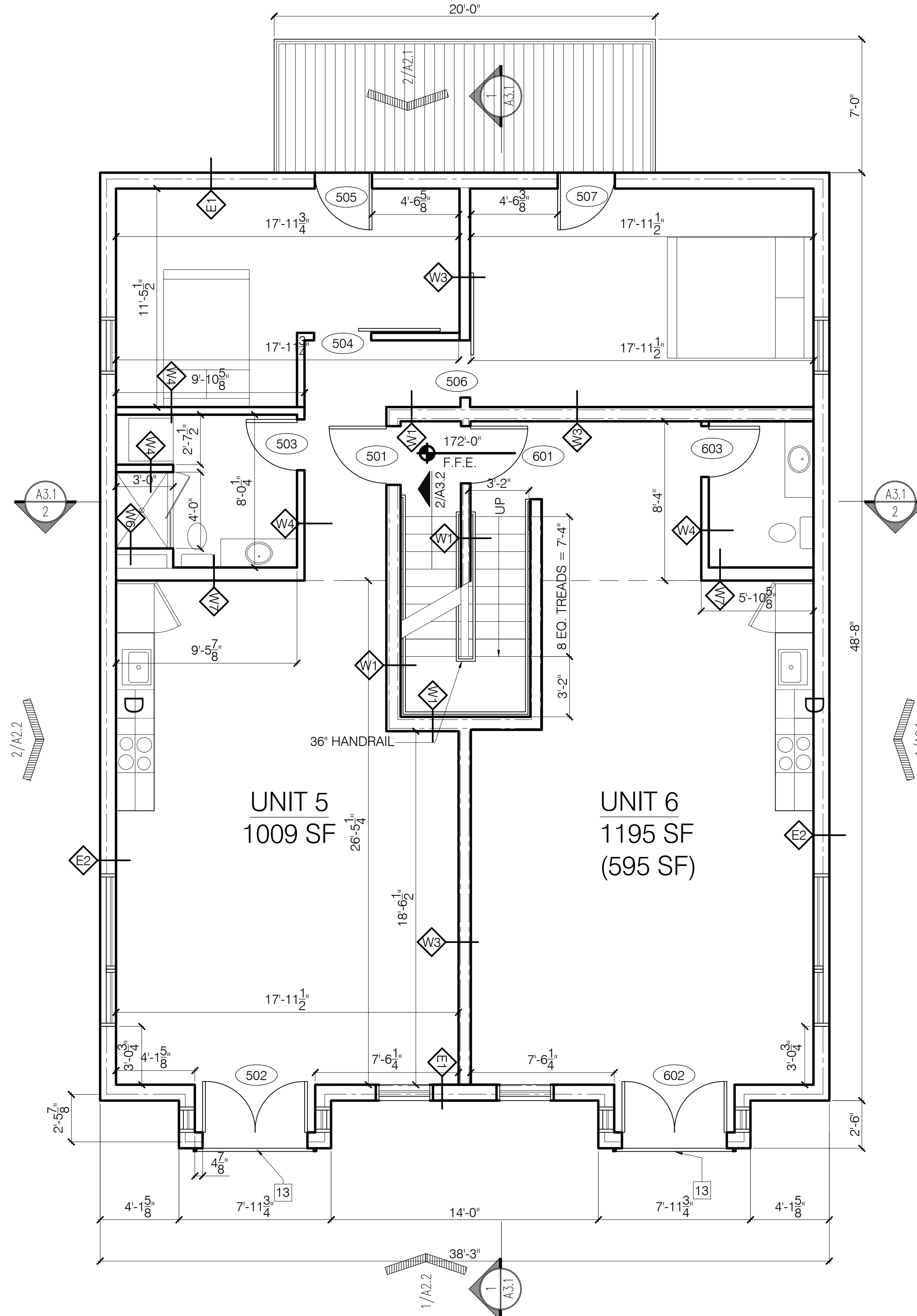
THIRD FLOOR SCALE: 1/4" = 1'-0"
