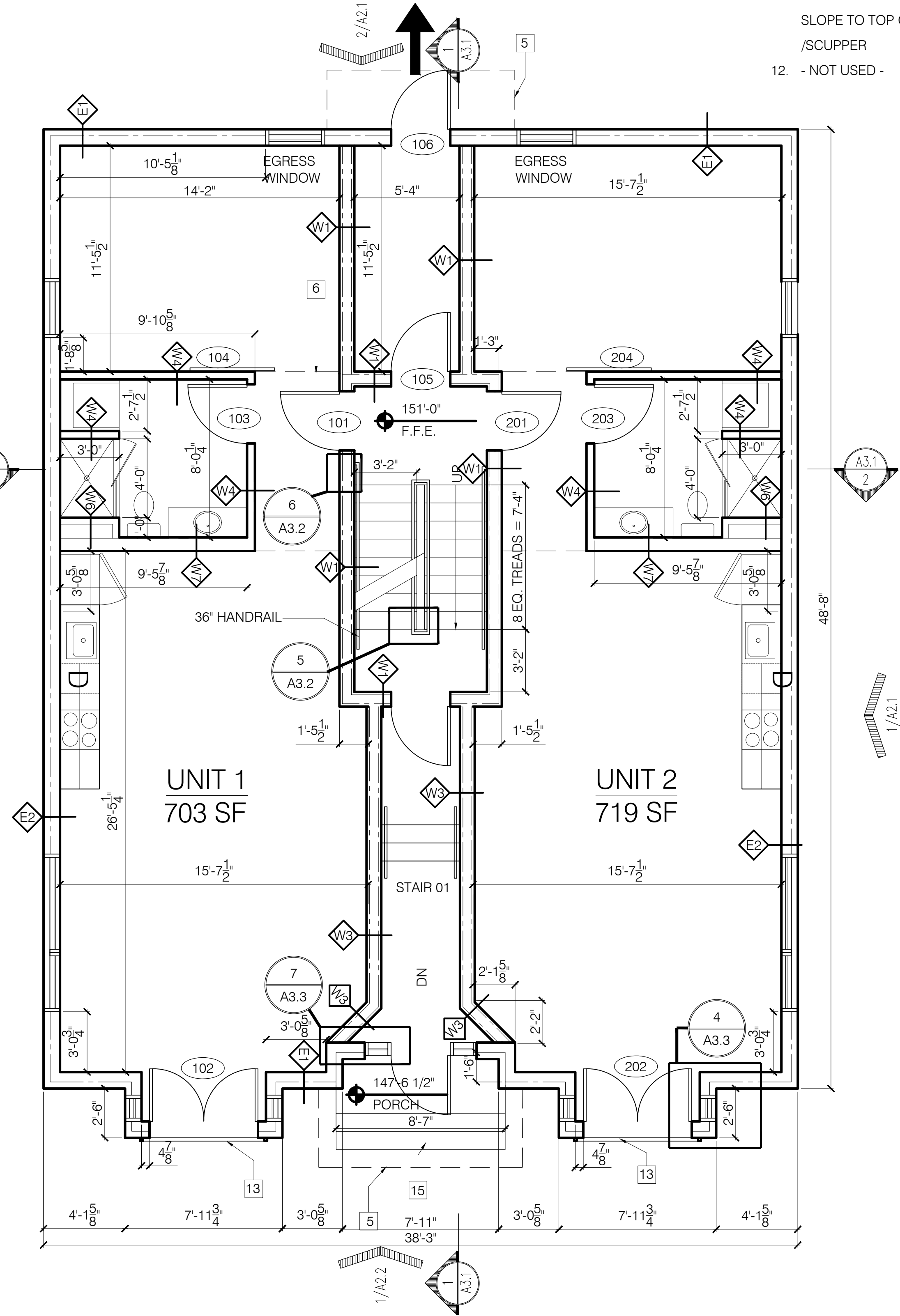
2 FIRST FLOOR
