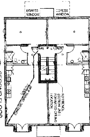
SECOND FLOOR SCALE: 1/8" = 1'-0"
