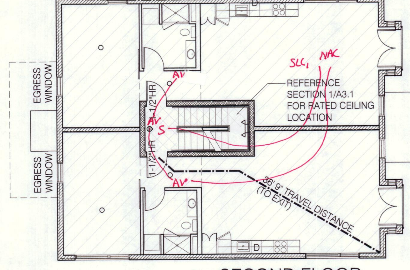
3 SECOND FLOOR SCALE: 1/8" = 1'-0"
