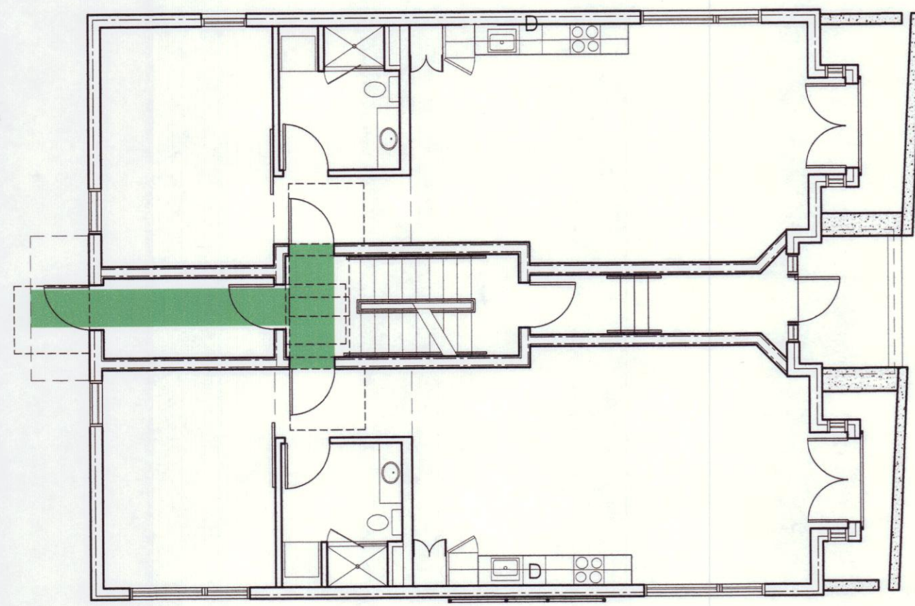
7 FIRST FLOOR ACCESSIBLE ROUTE SCALE: 1/8" = 1'-0"
