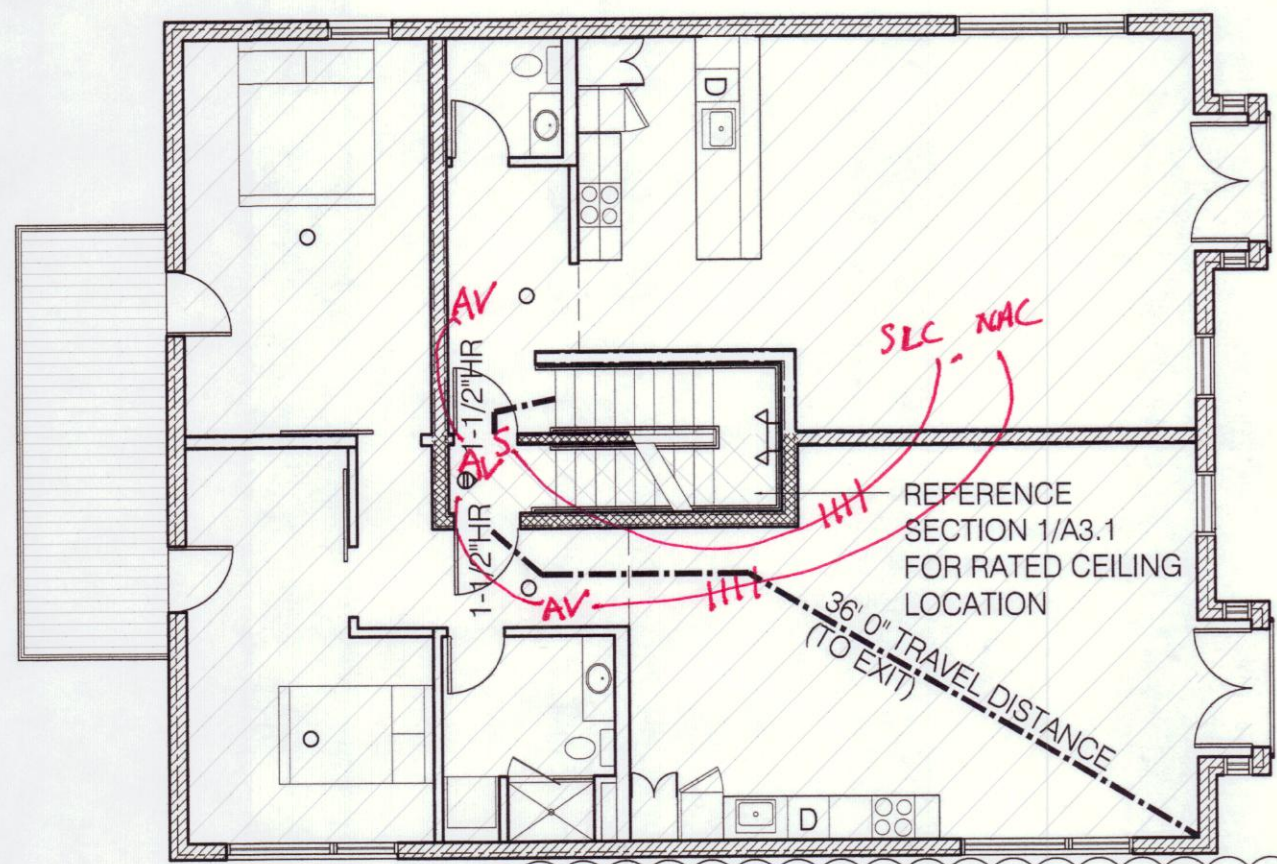
4 THIRD FLOOR SCALE: 1/8" = 1'-0"
