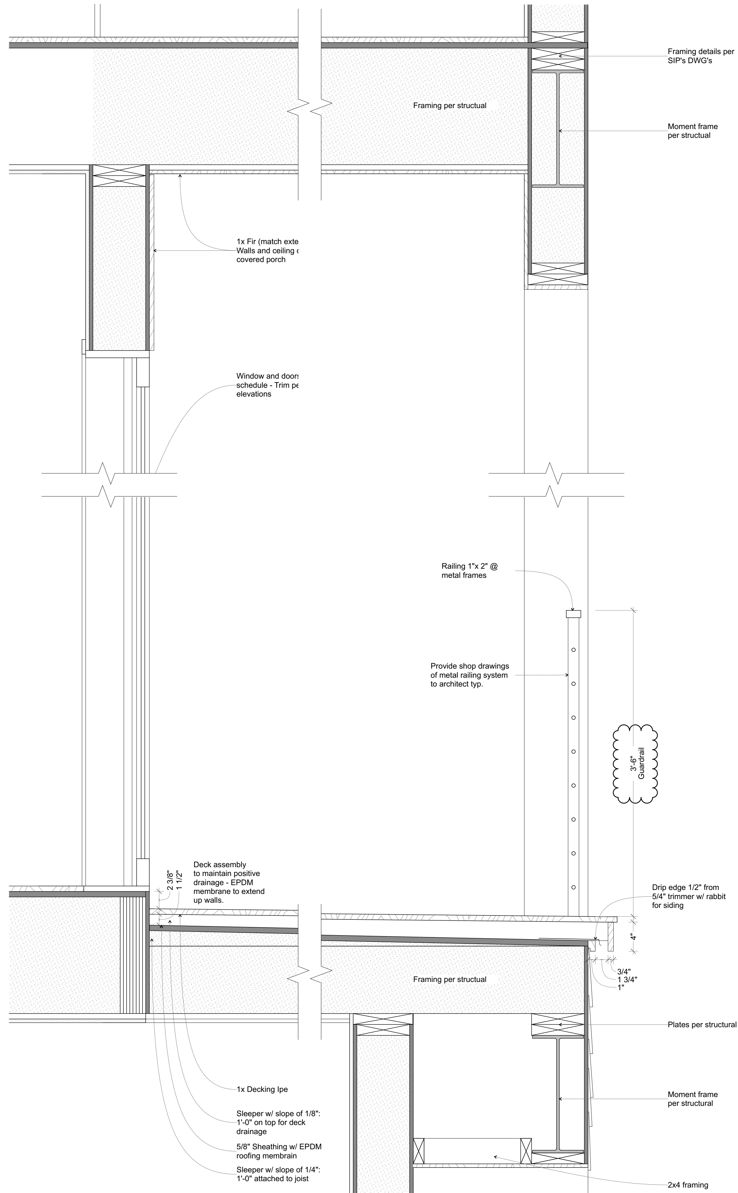
1 Covered Deck SCALE: 1 1/2" = 1'-0"
