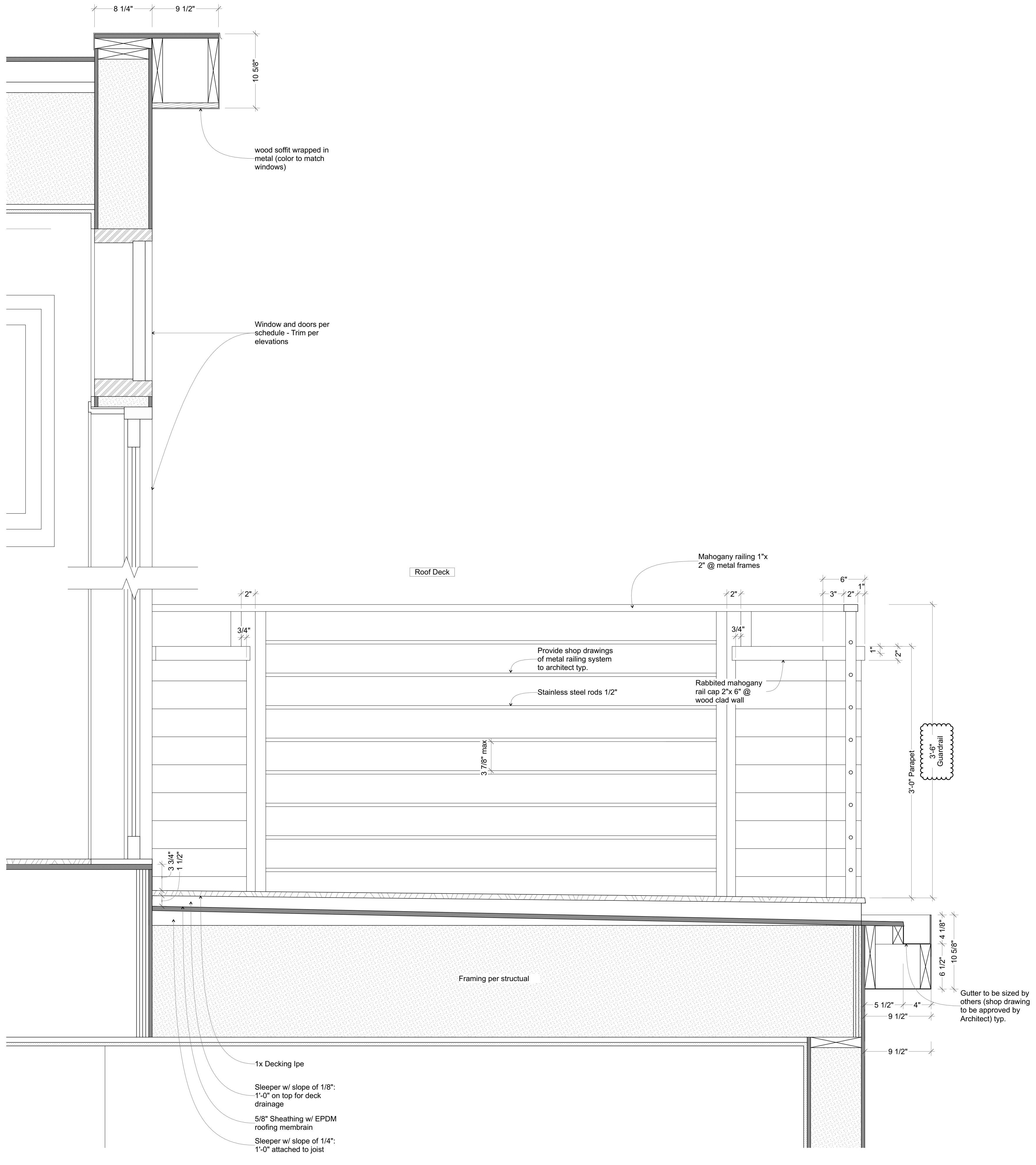
2 Roof Deck SCALE: 1 1/2" = 1'-0"
