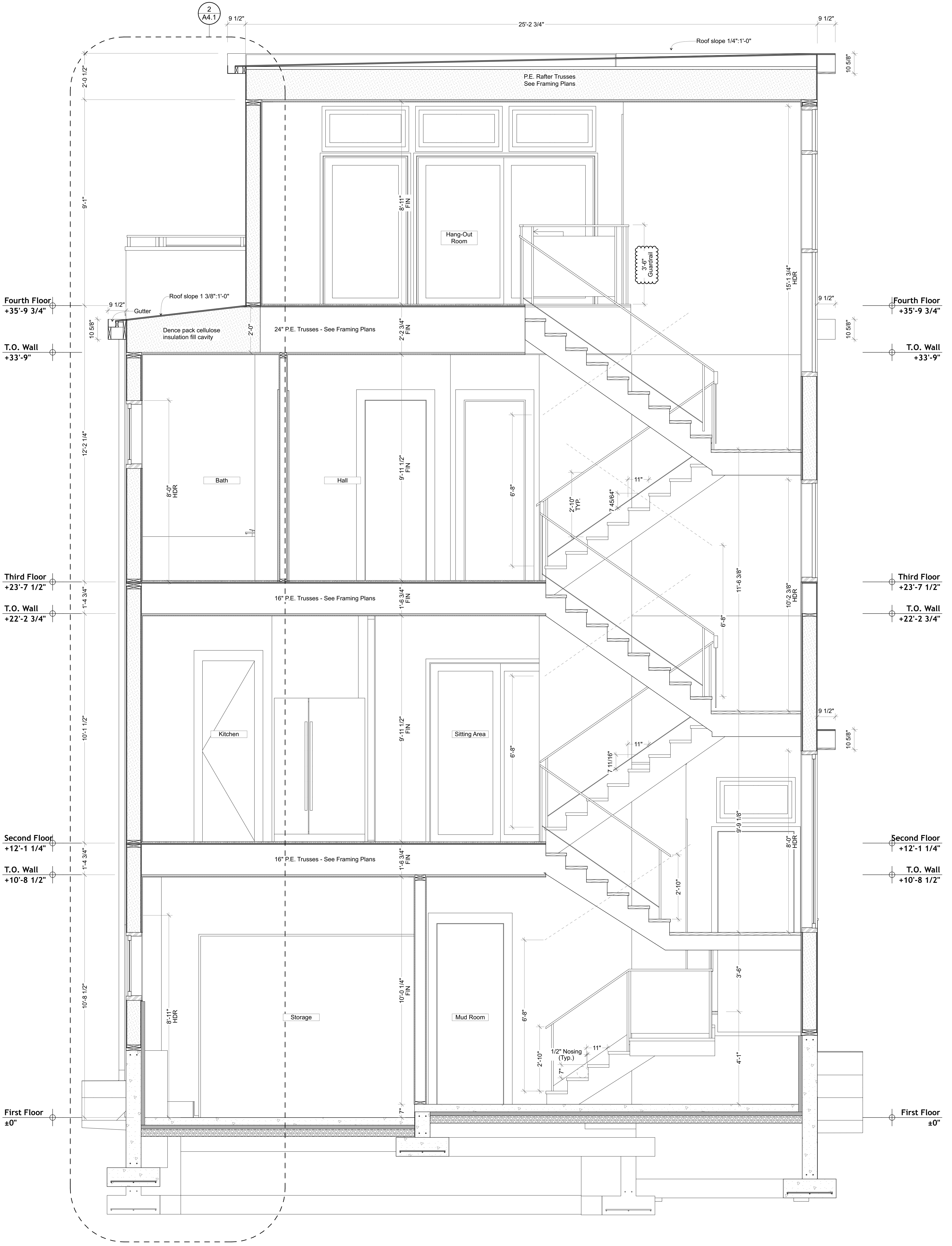
1 Section House N/S
