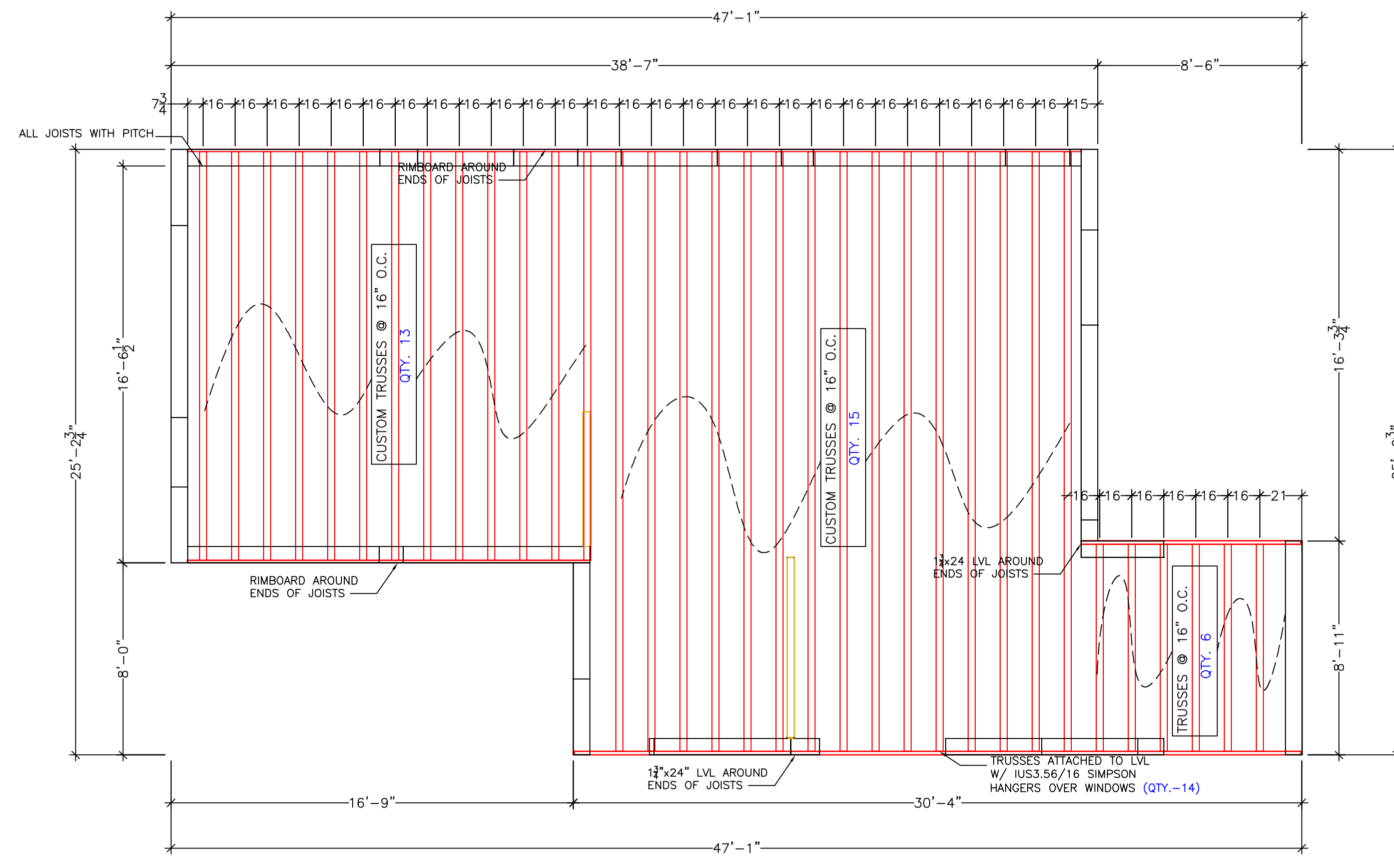
ROOF JOIST LAYOUT SCALE: 1/4" = 1'-0" (2)
