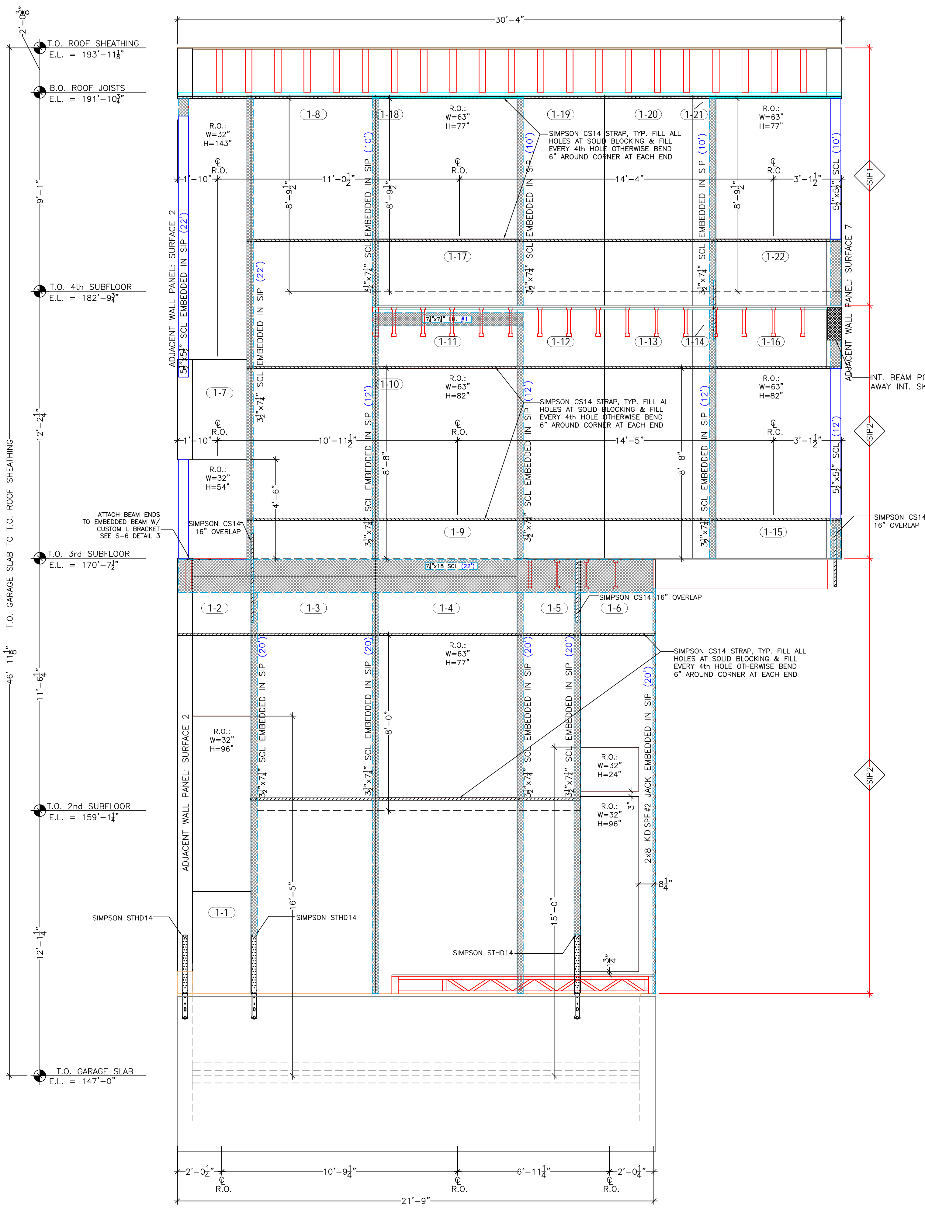
WALL PANEL LAYOUT: SURFACE 1 SCALE: 3/8" = 1'-0" [PANEL SPEC: 8 1/4" EPS SIP]
