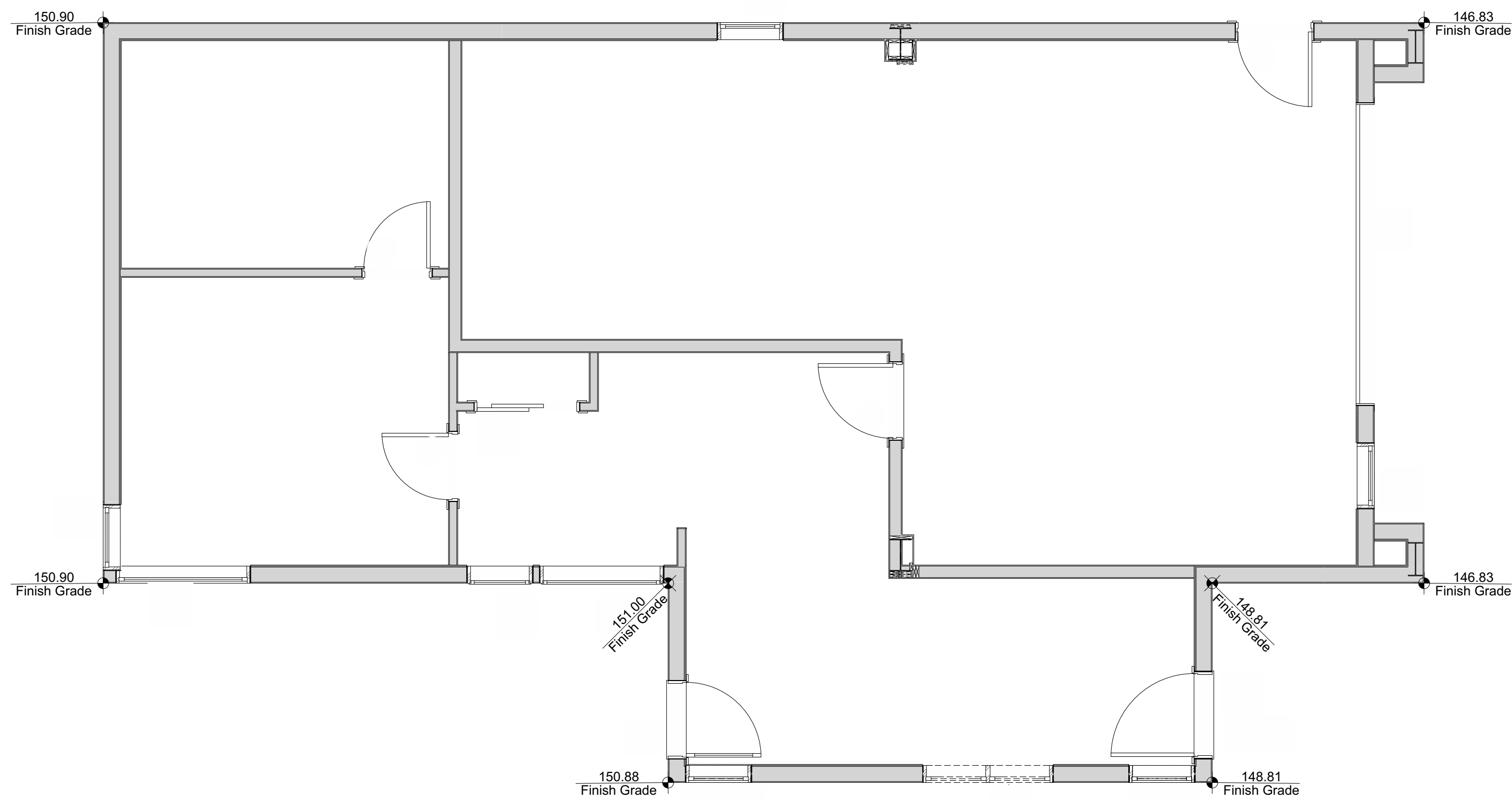
1 Finish Grade Elevation Plan SCALE: 1/4" = 1'-0"
