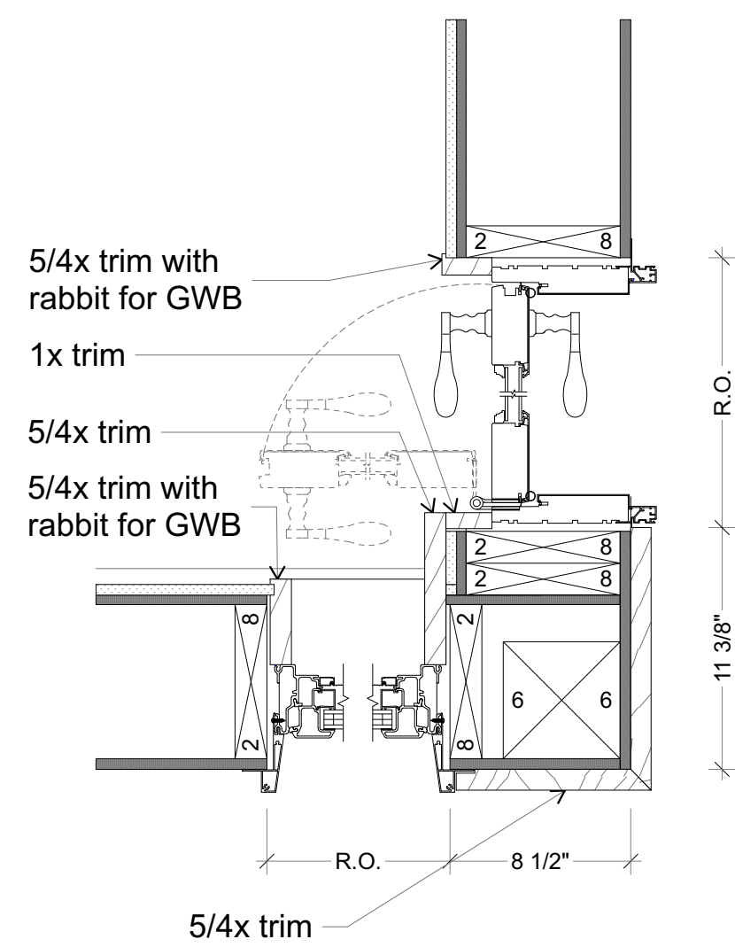
2 Entry Door & Window - Plan Detail SCALE: 1 1/2" = 1'-0"
