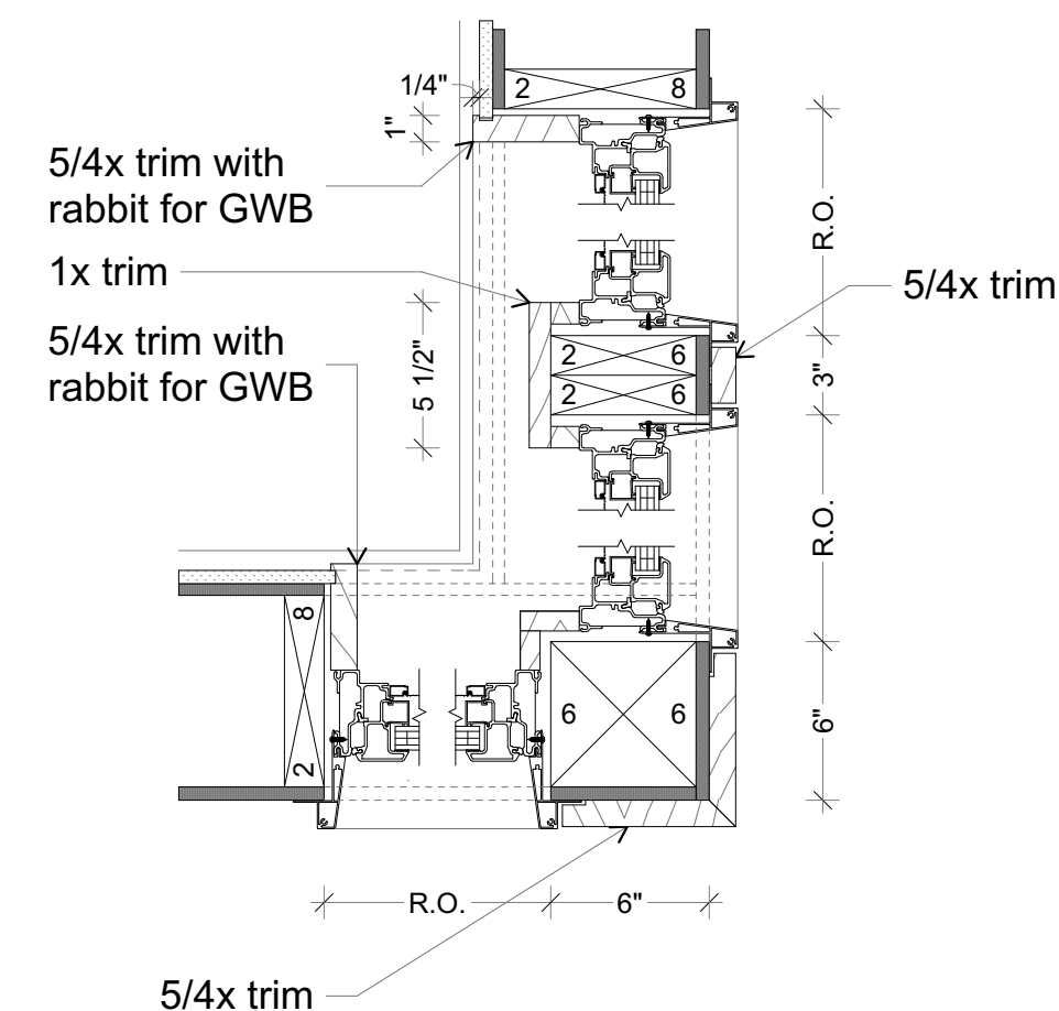
3 Corner Window - Plan Detail SCALE: 1 1/2" = 1'-0"
