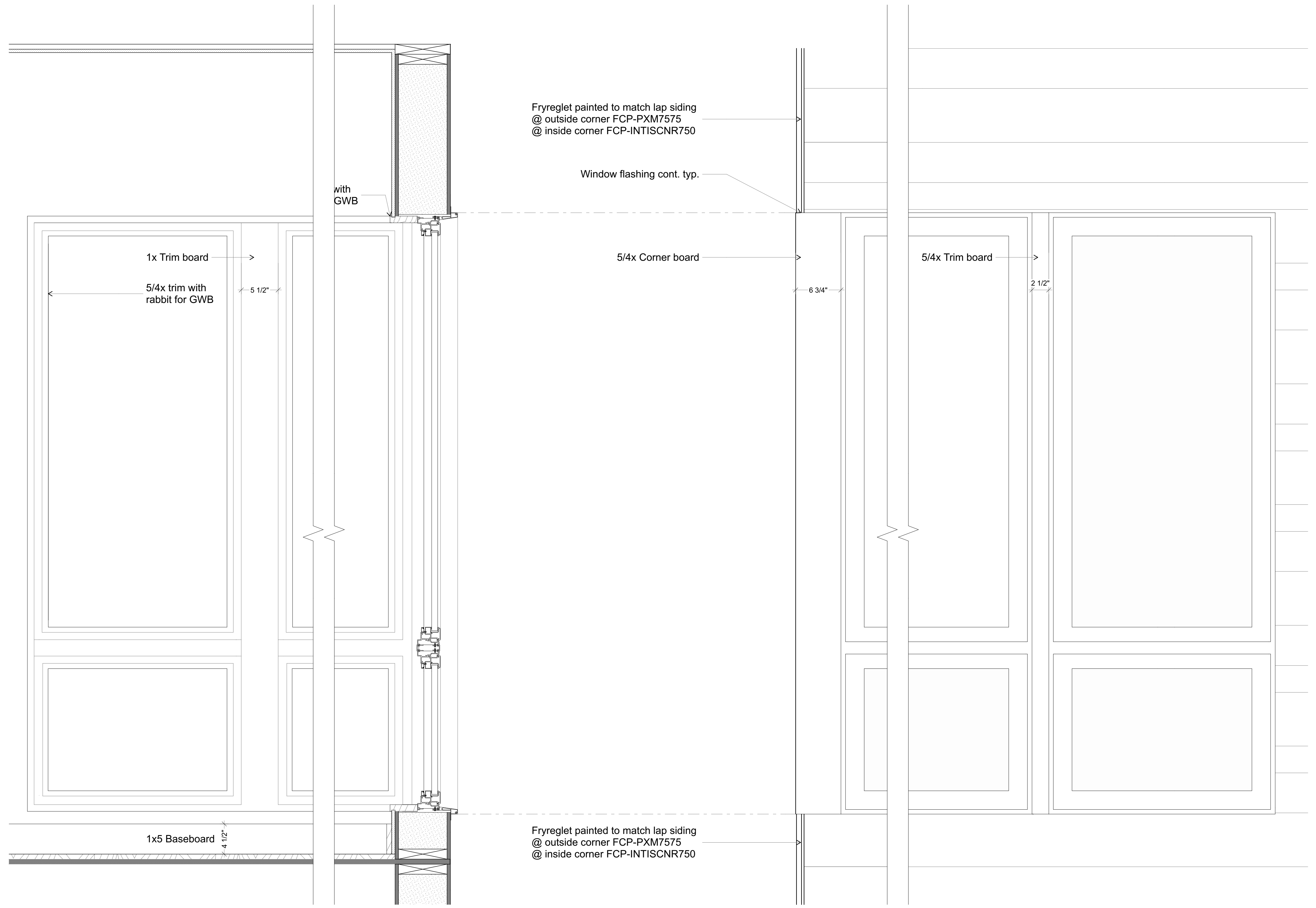
4 Interior & Exterior Trim Typical SCALE: 1 1/2" = 1'-0"
