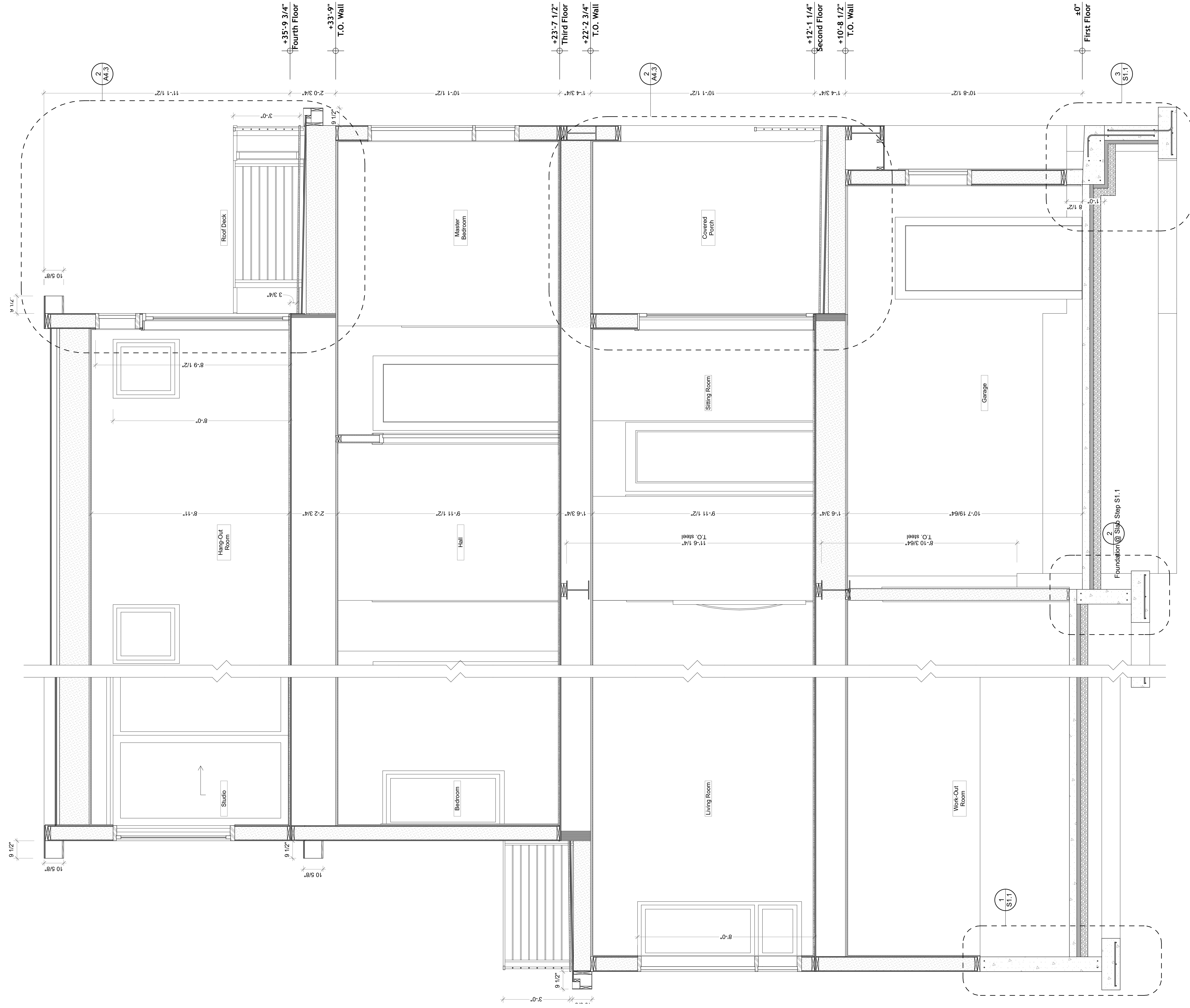
2 Section House E/W SCALE: 1/2" = 1'-0"
