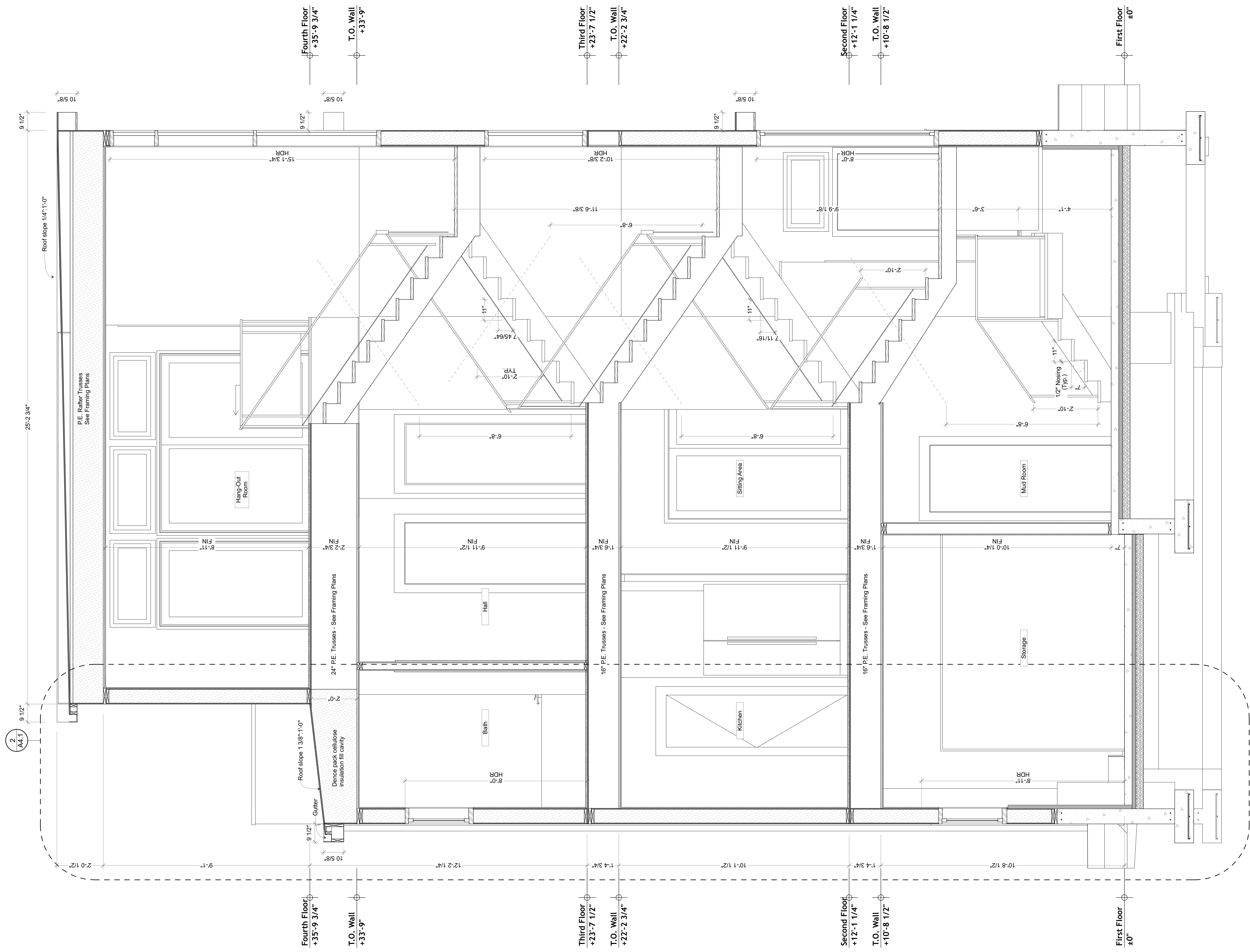
1 Section House N/S SCALE: 1/2" = 1'-0"
