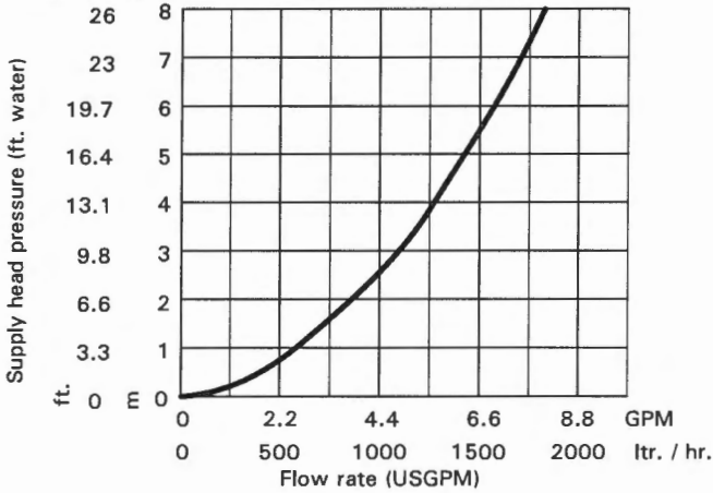
Pressure drop (primary circuit) of Vitodens 100-W
