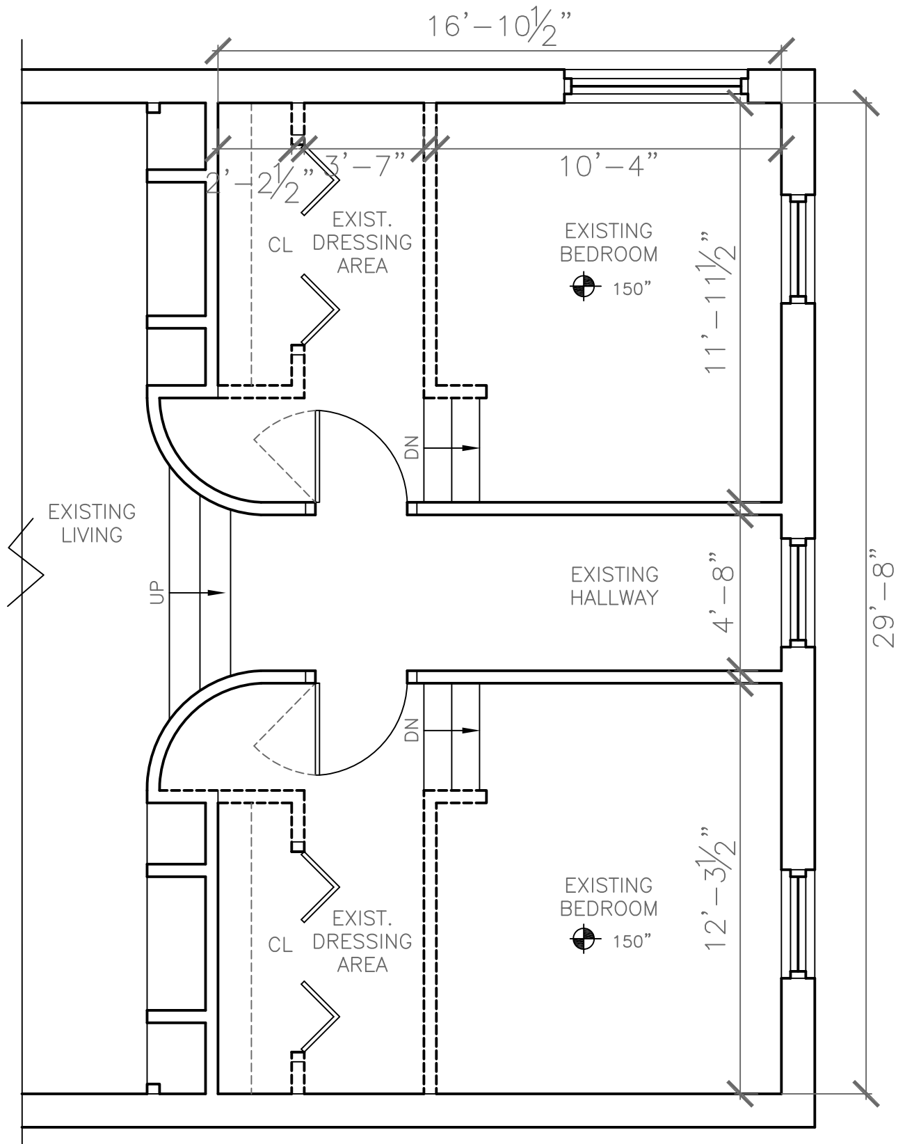
(A) Existing Bedroom Floor Plan 1/4" = 1'-0"
