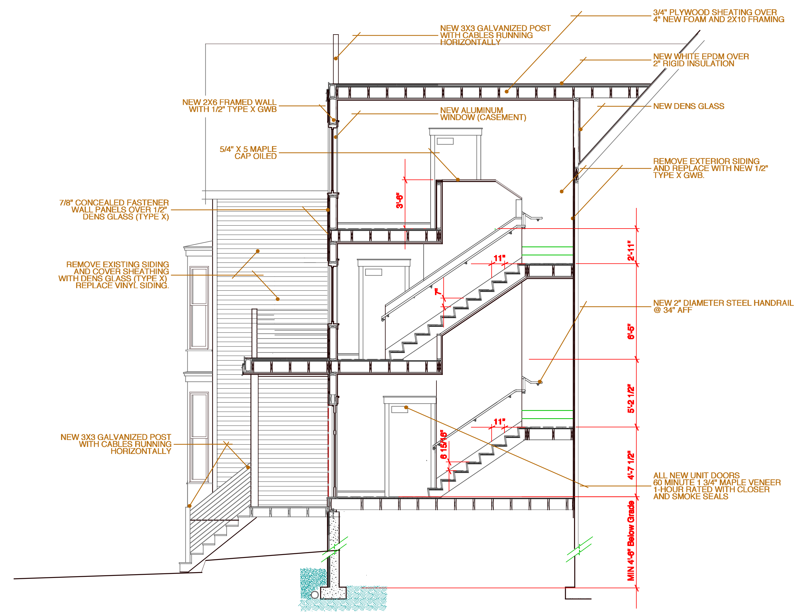
10 Section at Stair 0 2 6 12
