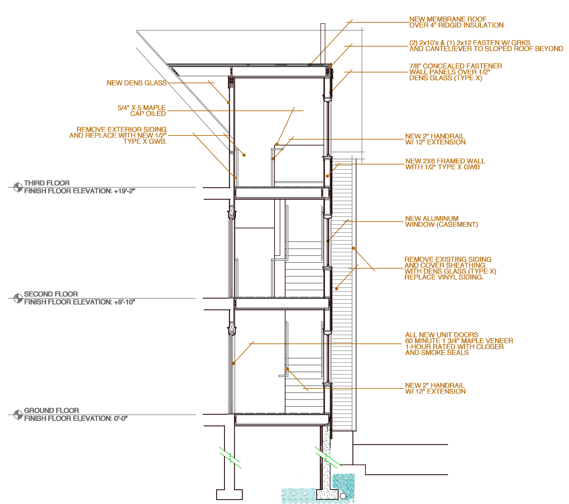
20 Cross Section at Stair 0 2 6 12
