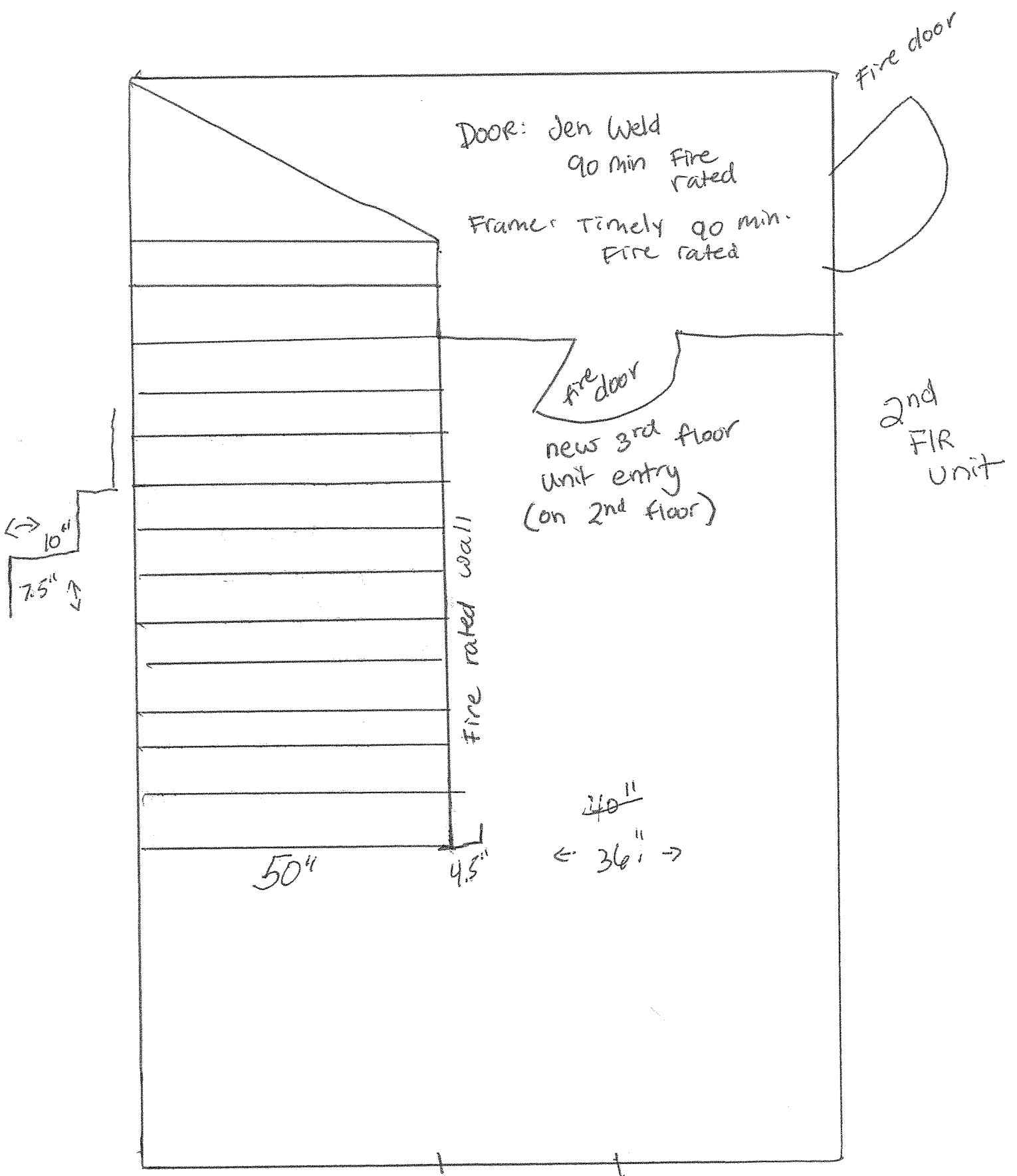
Proposed 2nd FIR HALL / STAIR (work area detail)
