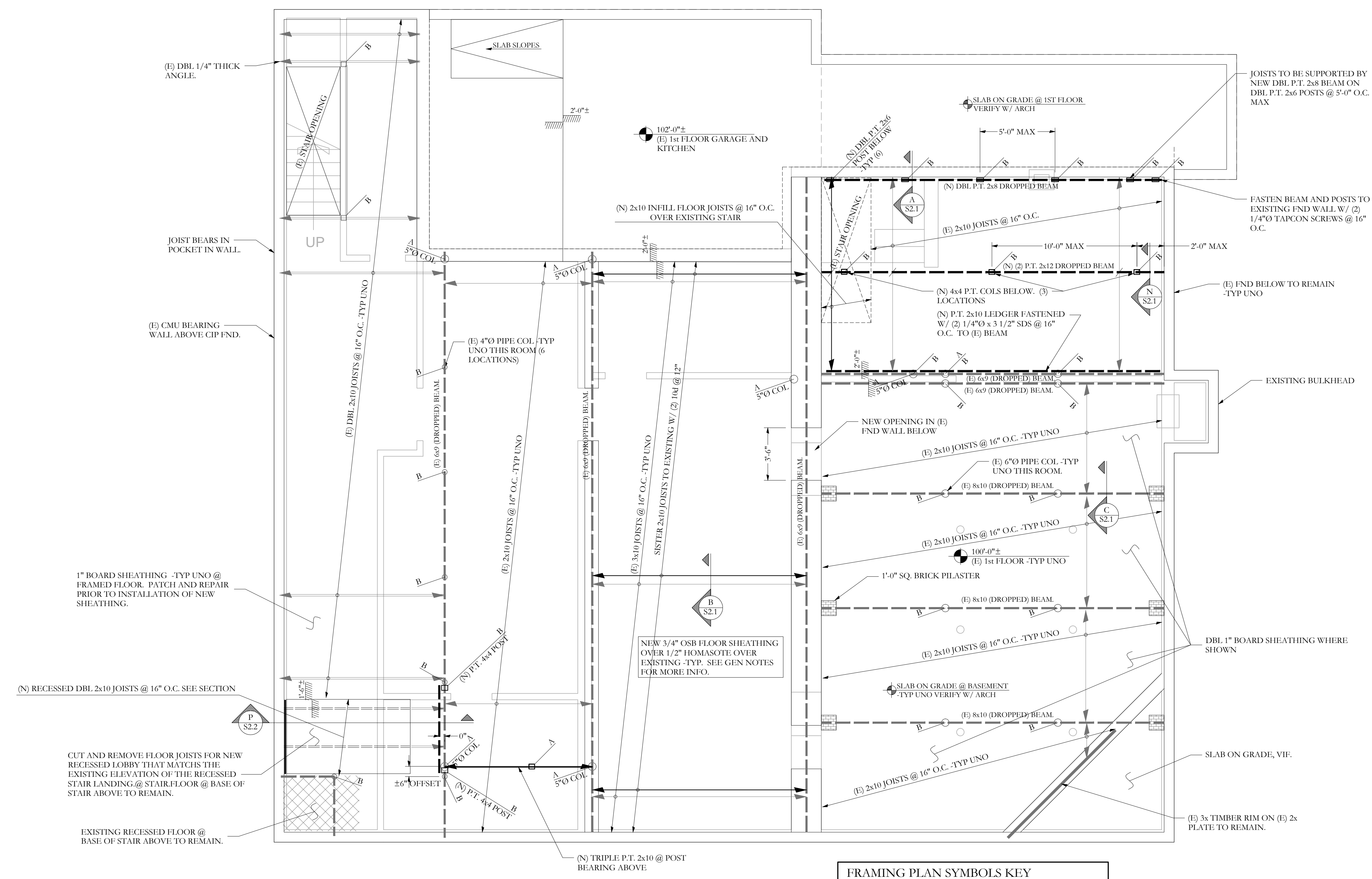
MAIN LEVEL FRAMING PLAN SCALE 1/4"=1'-0"
