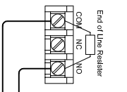
OSYSU-2 Outside Screw and Yoke Valve Supervisory Switch
