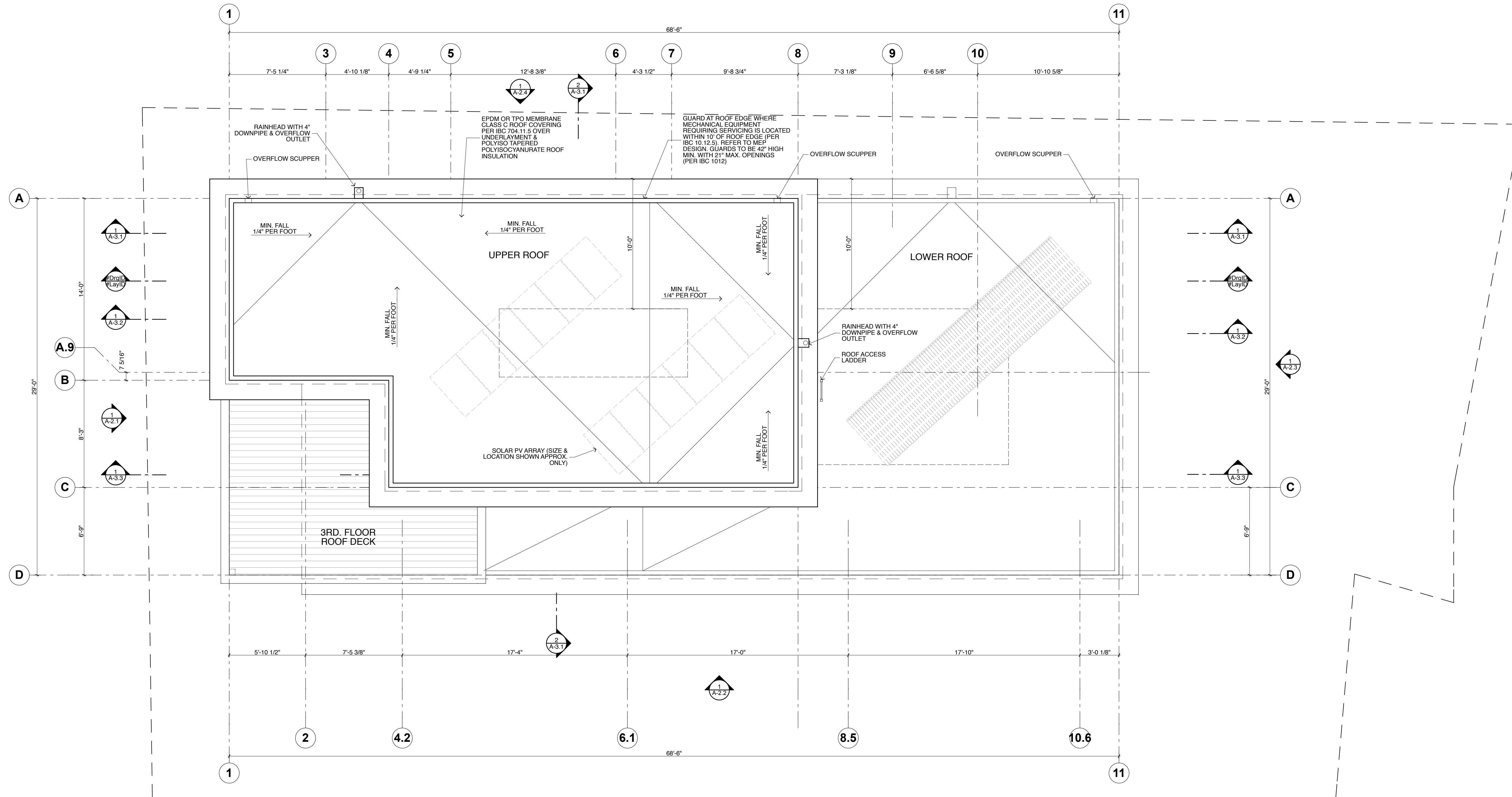
1 Roof SCALE: 1/4" = 1'-0"
