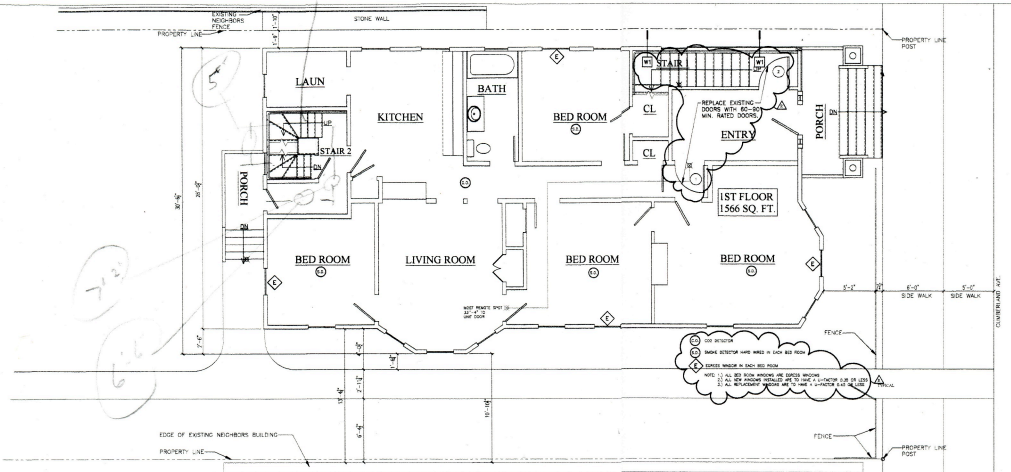
(N1) FIRST FLOOR EXISTING & PROPOSED
