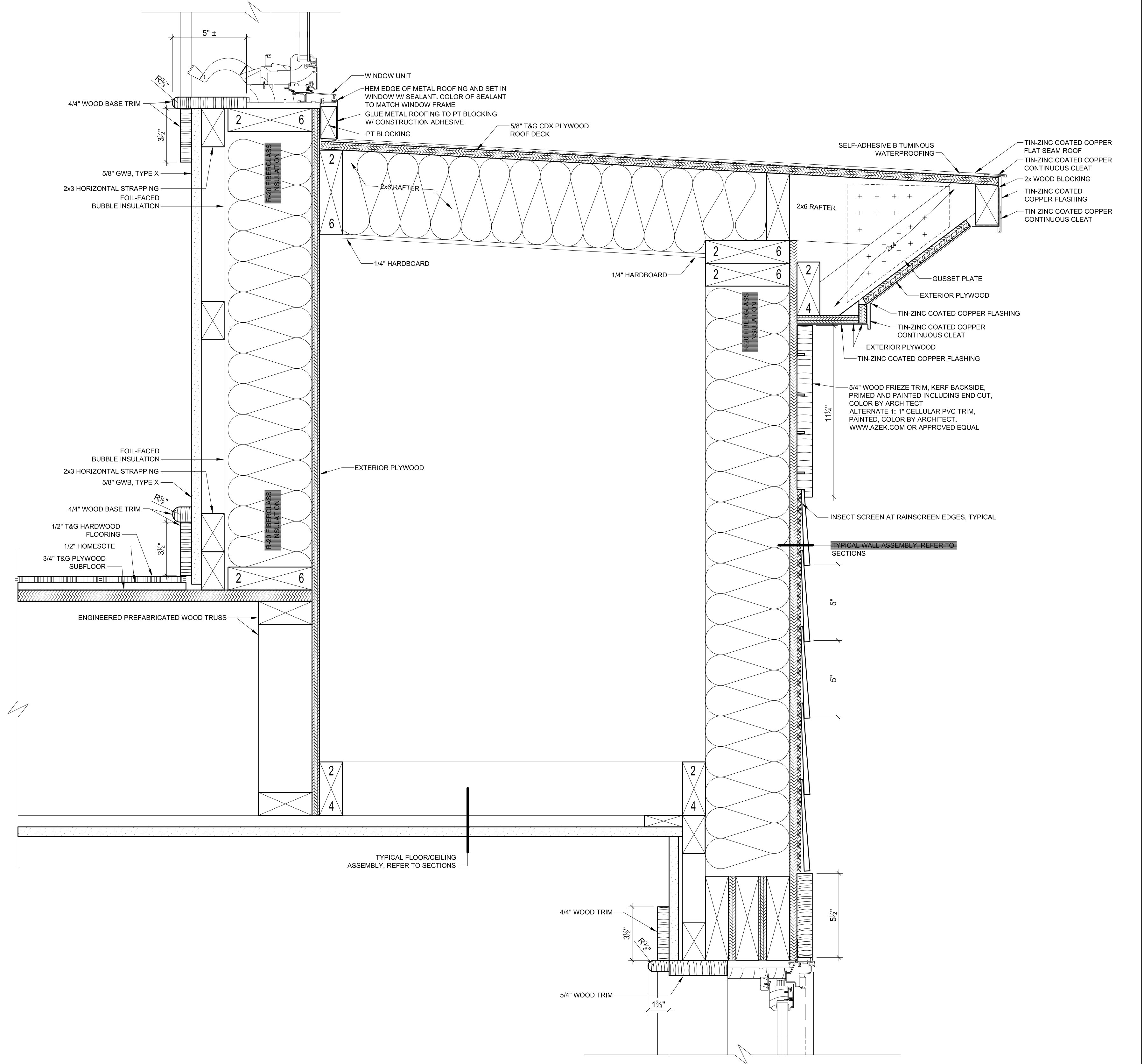
1 BAY WINDOW AT EAVE A4-4 SCALE: 3" = 1'-0"
