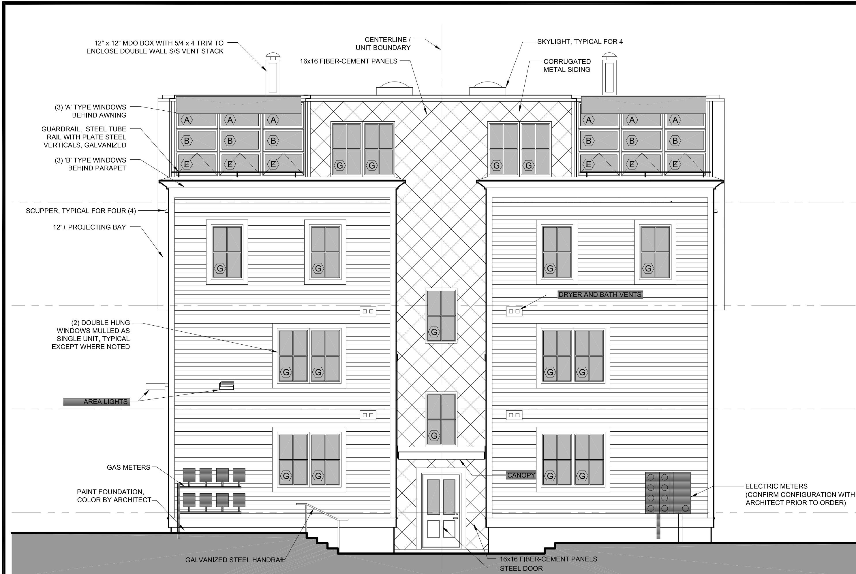
3 REAR (EAST) ELEVATION A2-1 SCALE: 3/16" = 1'-0"
