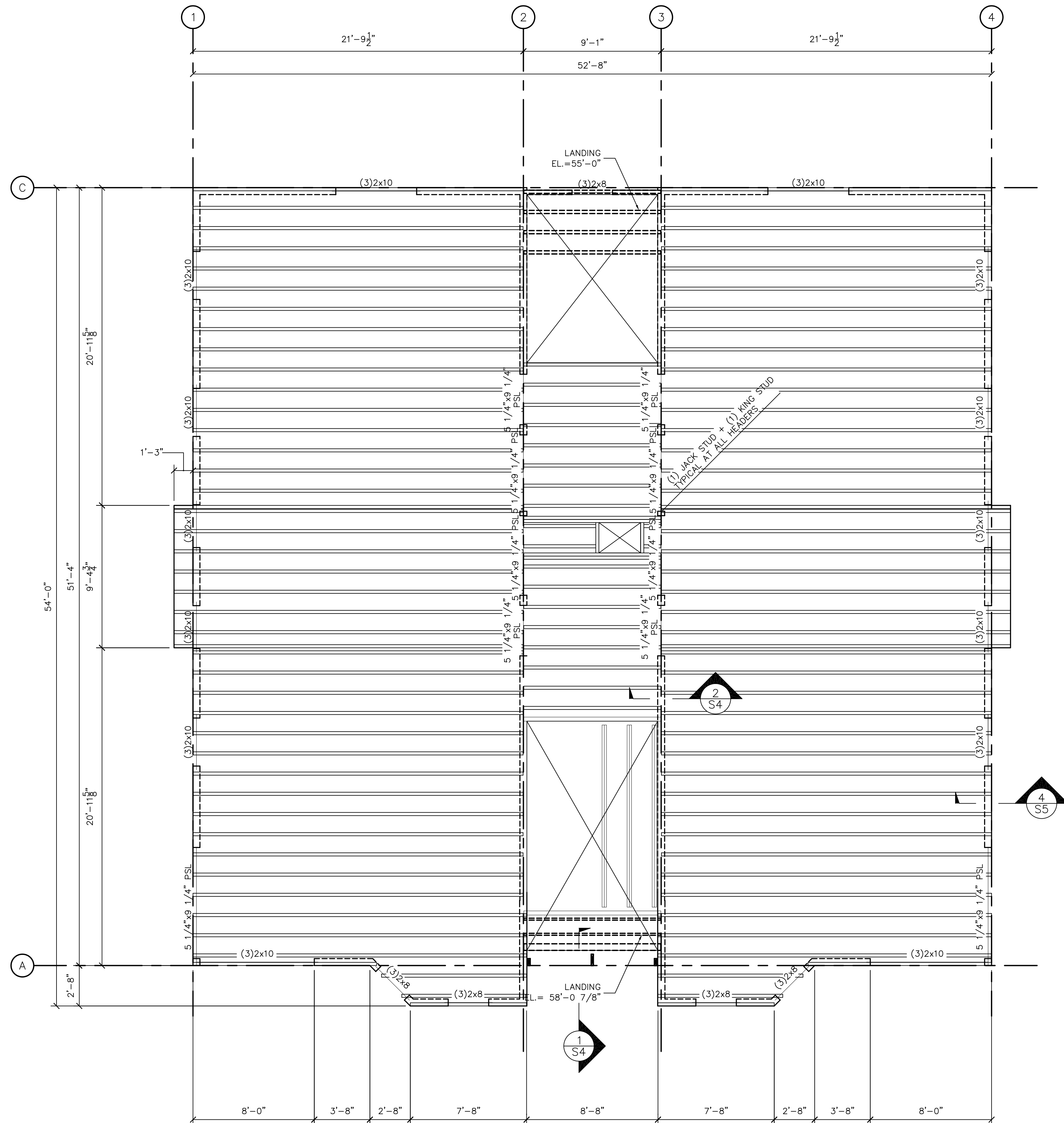
THIRD FLOOR FRAMING PLAN 1/4"=1'-0"
