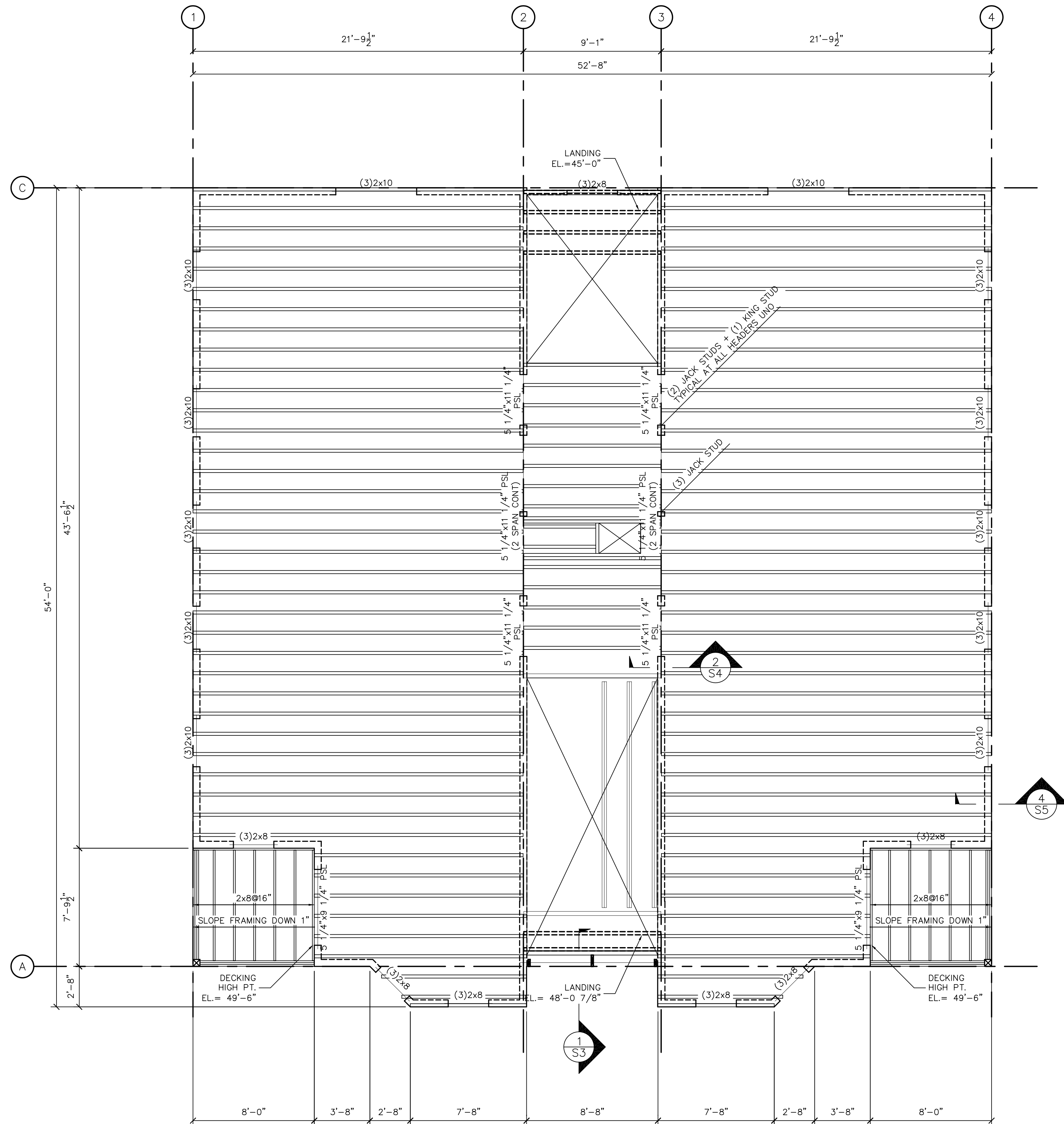
SECOND FLOOR FRAMING PLAN 1/4"=1'-0"
