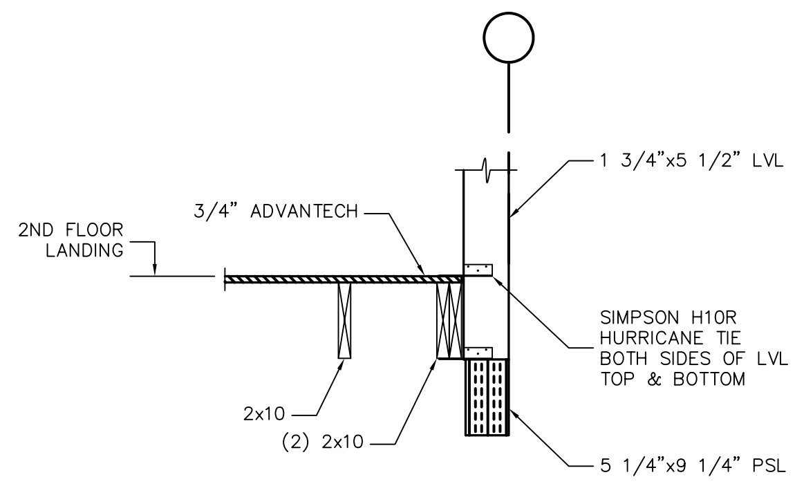
SECTION 1 3/4"=1'-0" S3
