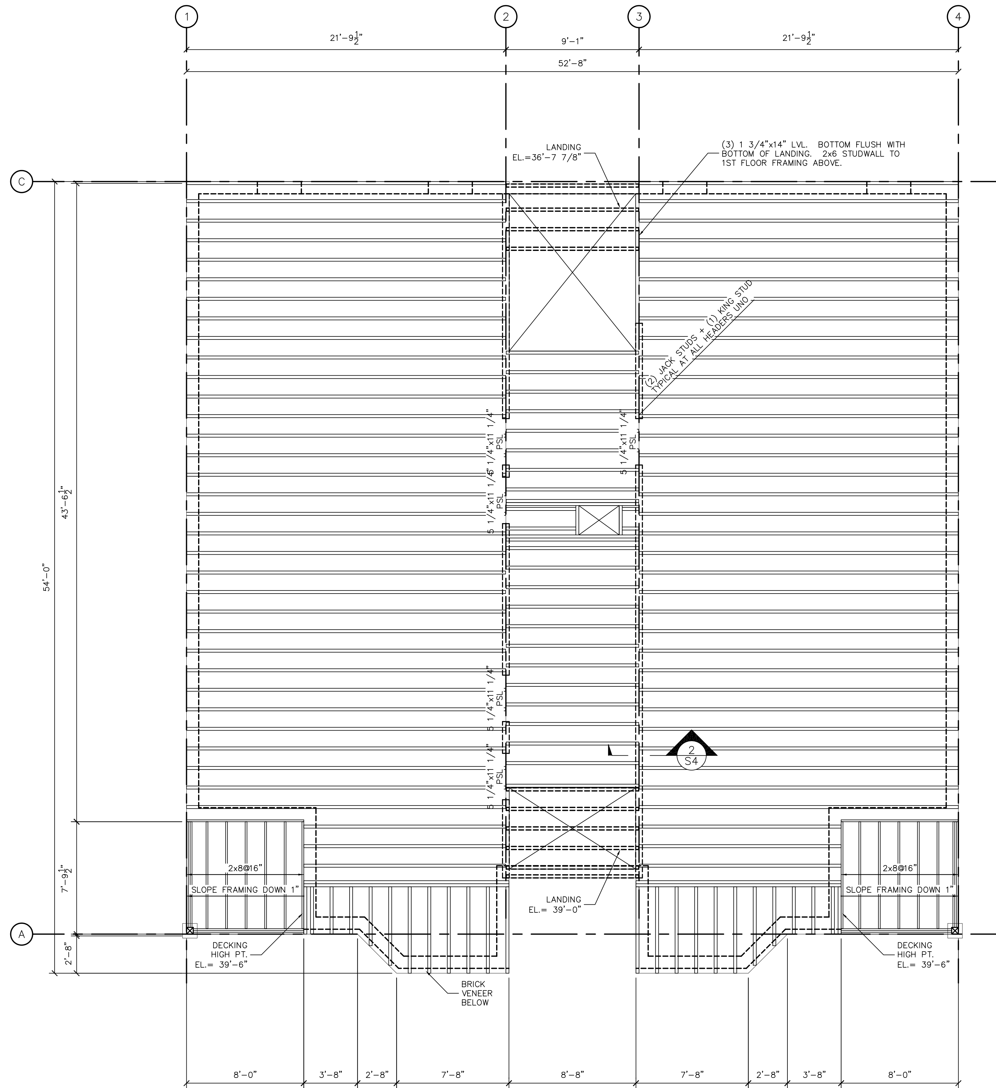
FIRST FLOOR FRAMING PLAN 1/4" = 1'-0"
