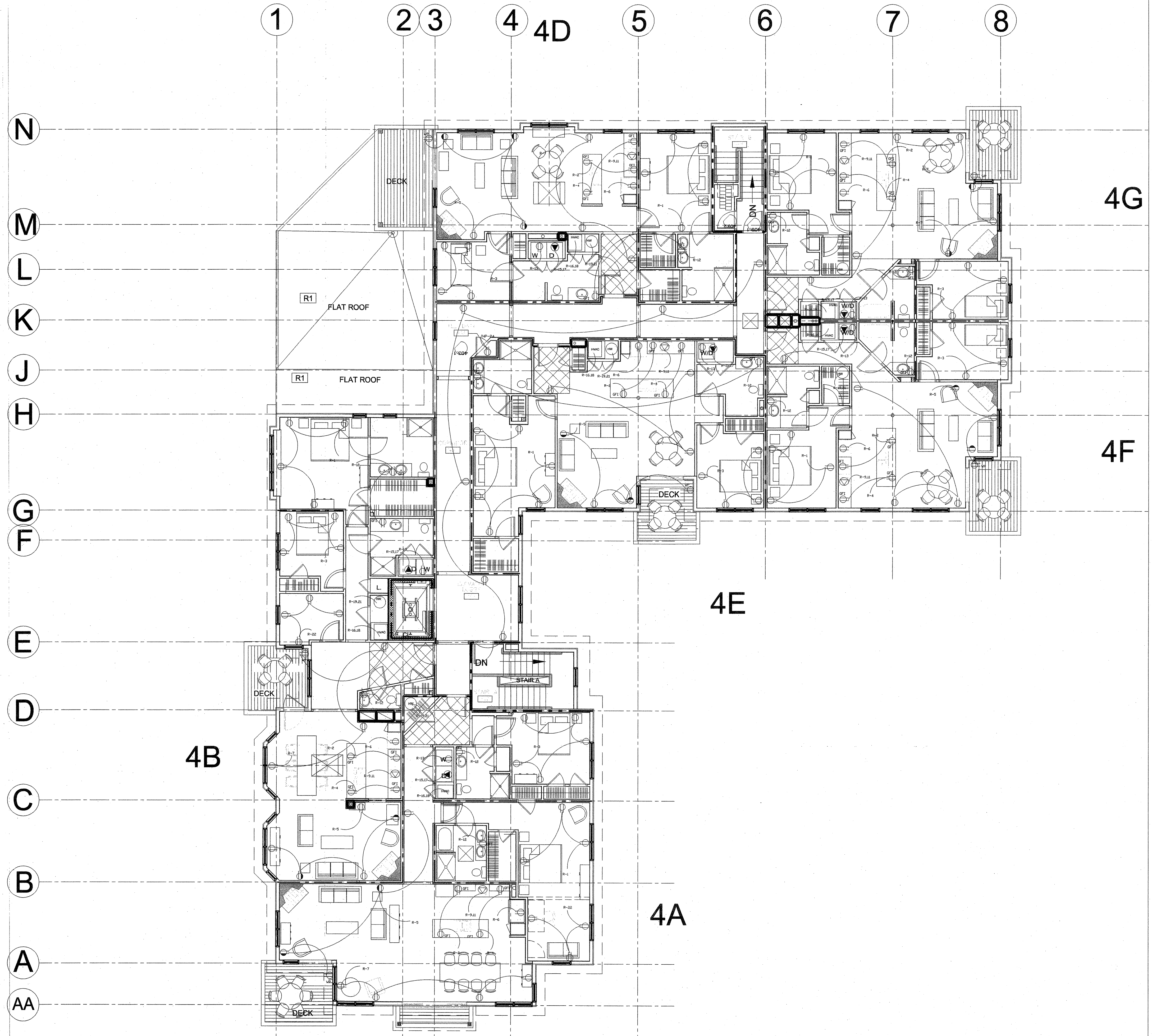
FOURTH FLOOR POWER PLAN 1/8" = 1'-0"
