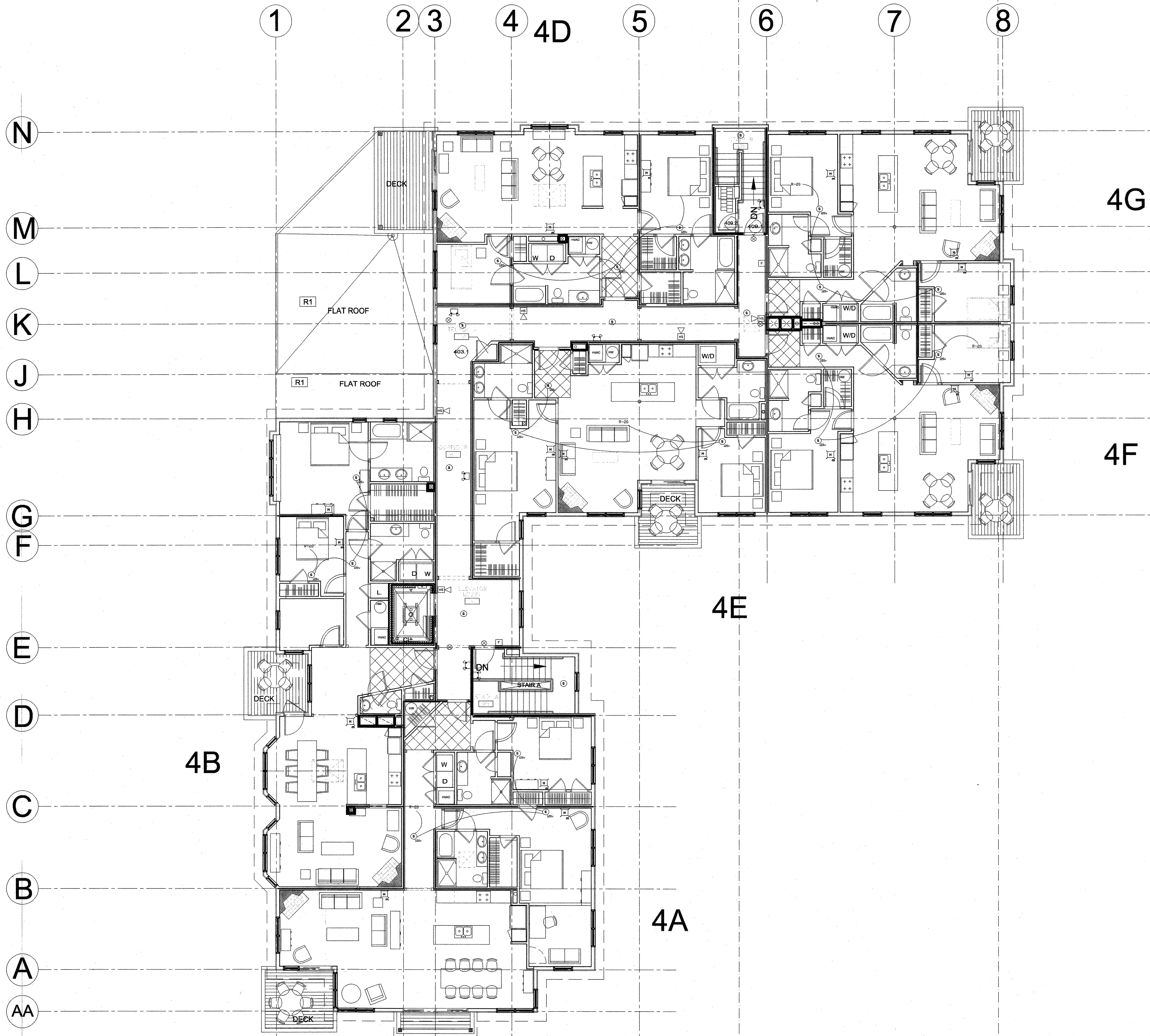
FOURTH FLOOR LIFESAFETY/ FIRE ALARM PLAN 1/8" = 1'-0"
