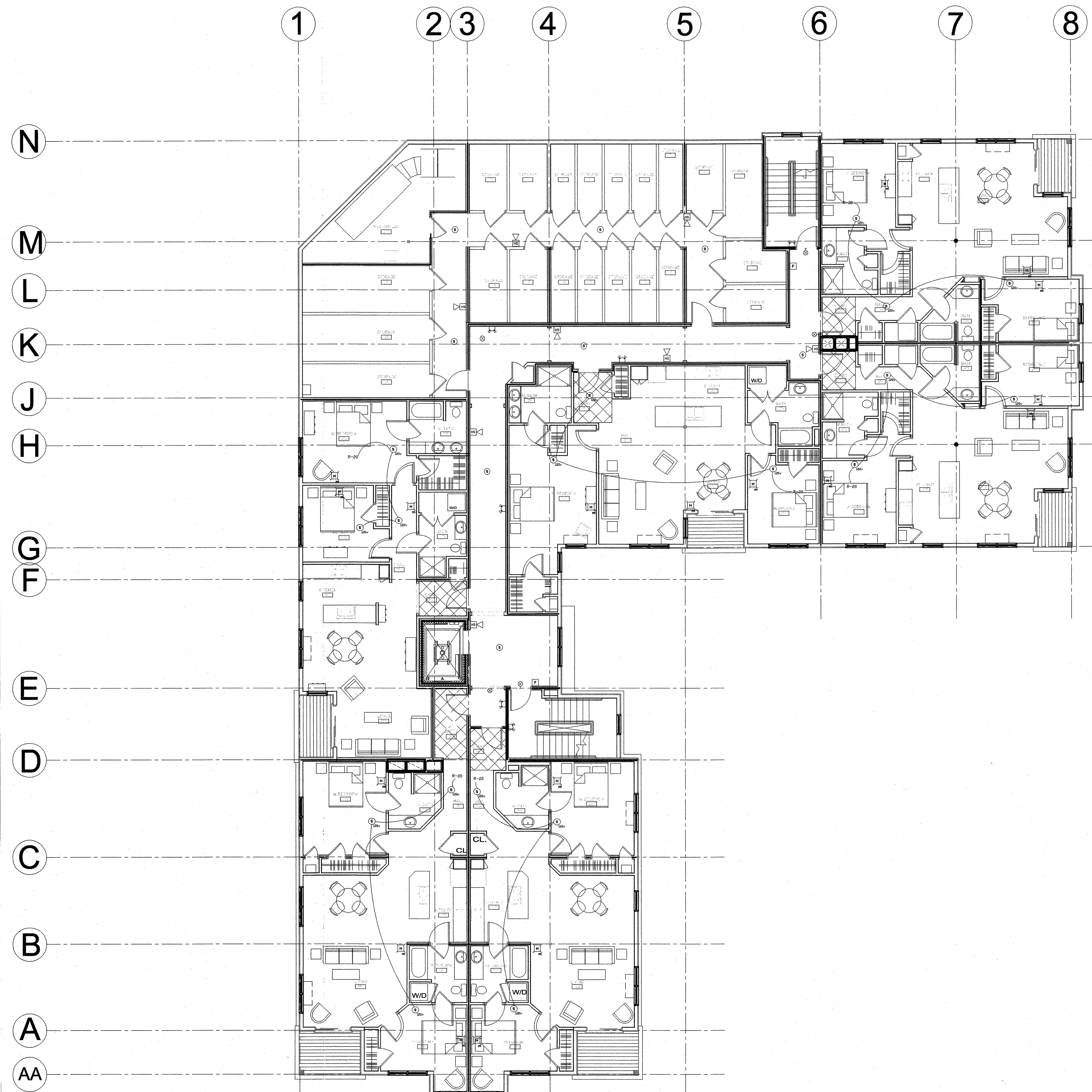
SECOND FLOOR LIFESAFETY/ FIRE ALARM PLAN 1/8" = 1'-0"
