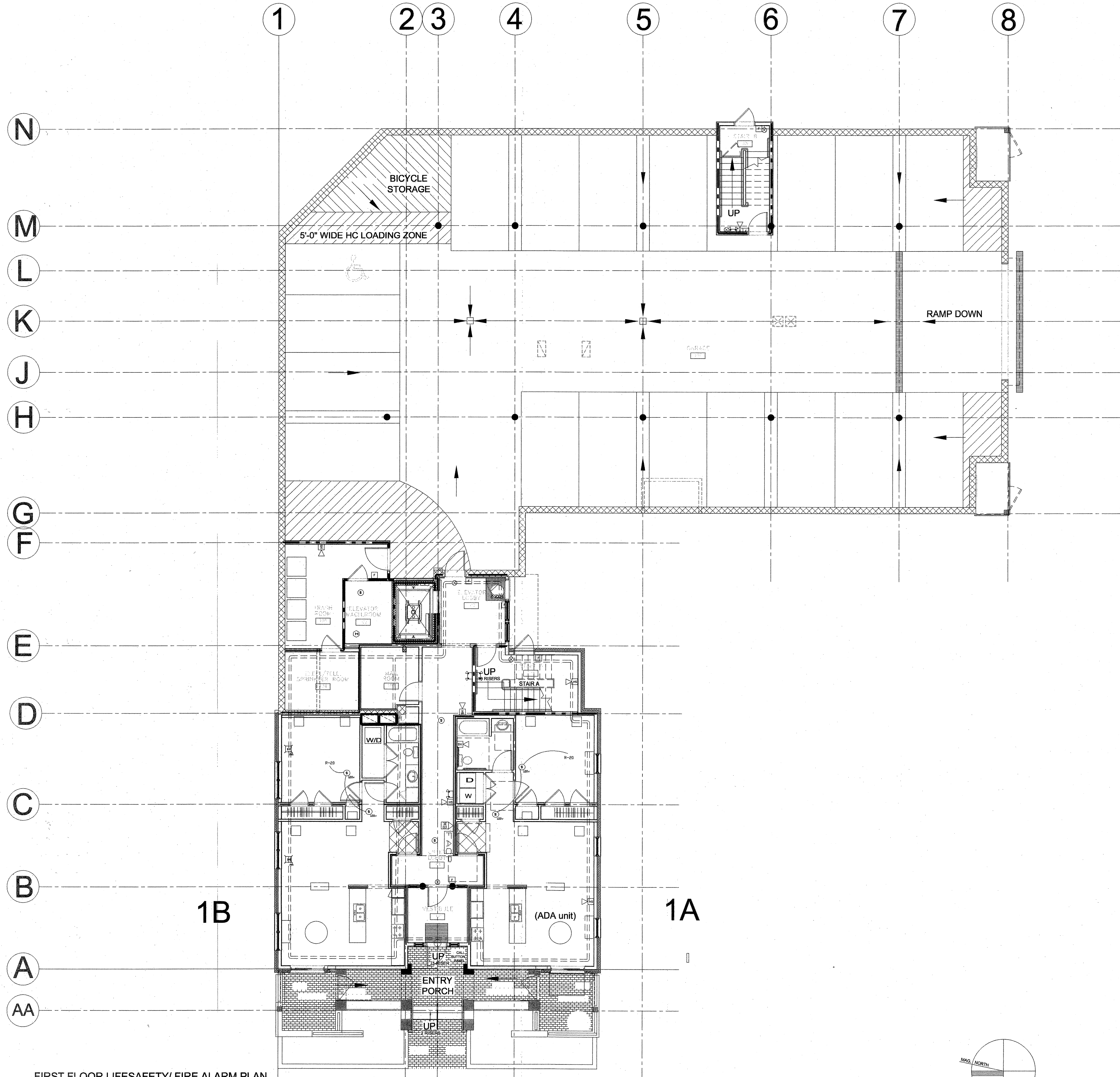
FIRST FLOOR LIFESAFETY/ FIRE ALARM PLAN 1/8" = 1'-0"
