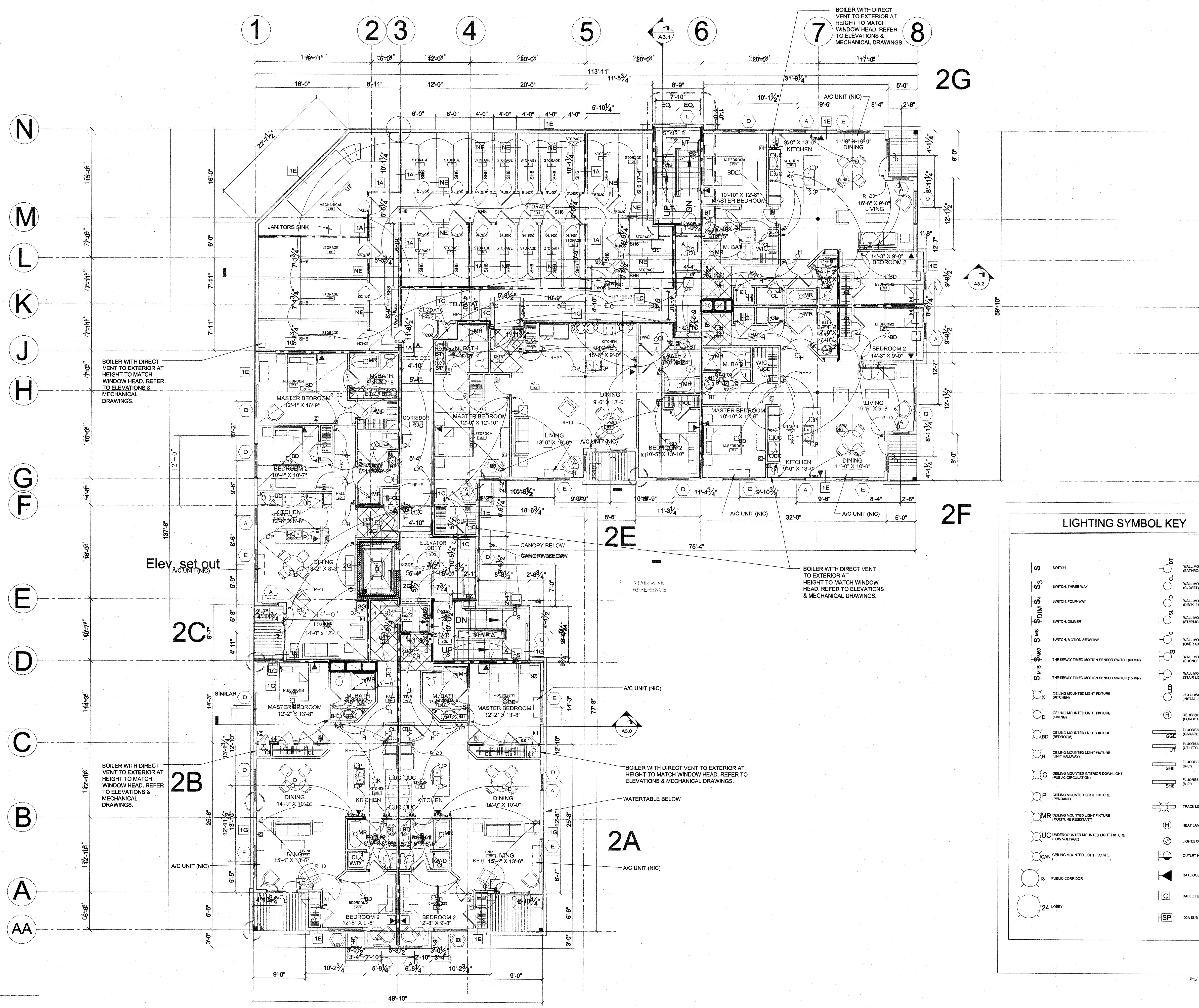
SECOND FLOOR LIGHTING PLAN A8.1
