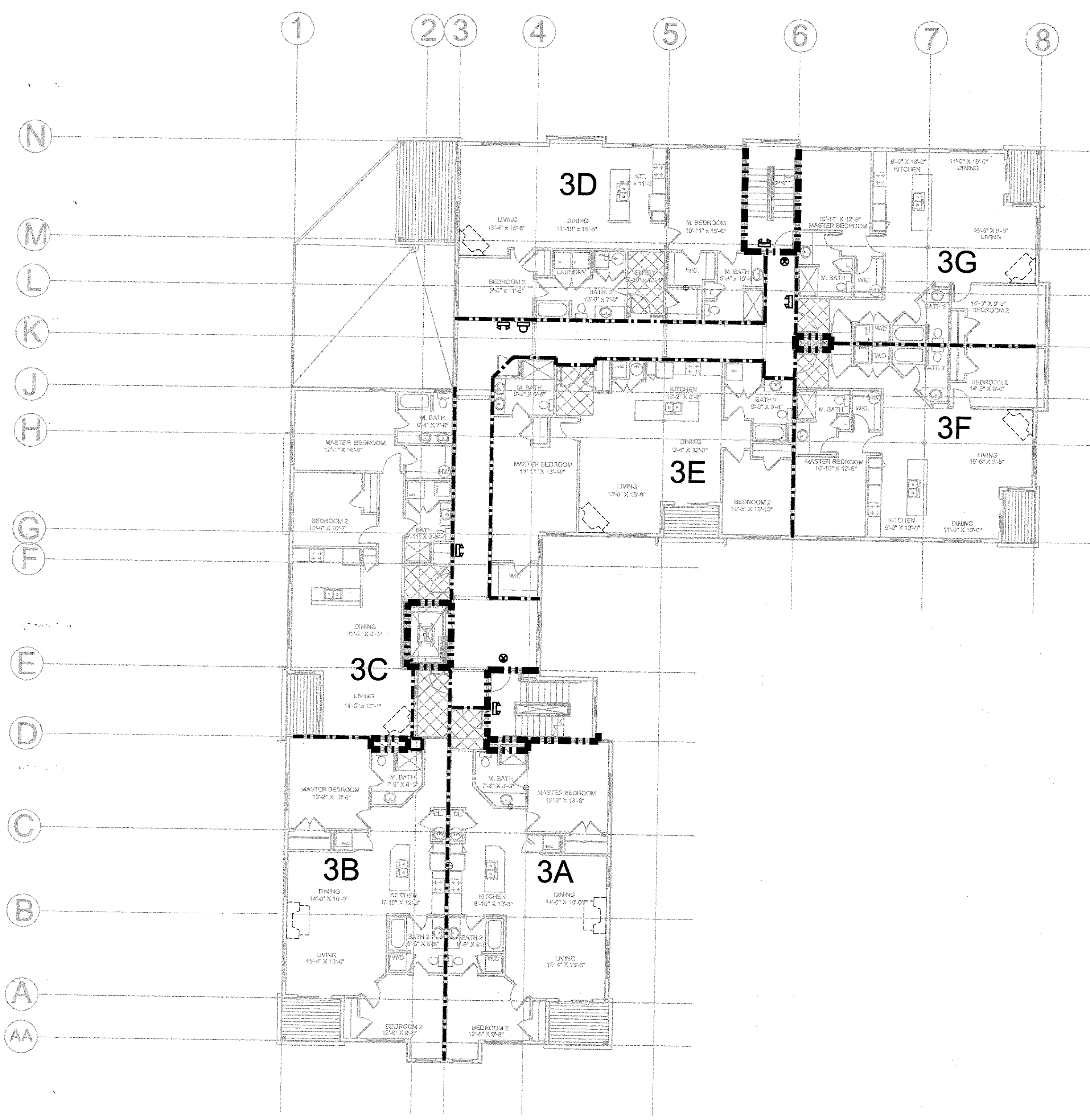
1 THIRD FLOOR LIFE SAFETY PLAN G1.3 3/32" = 1'-0"
