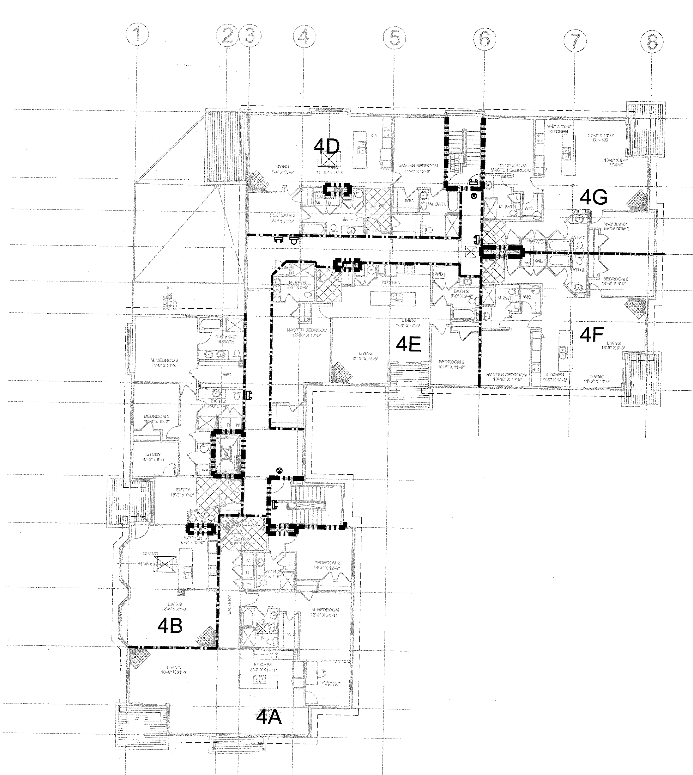
2 FOURTH FLOOR LIFE SAFETY PLAN G1.3 3/32" = 1'-0"
