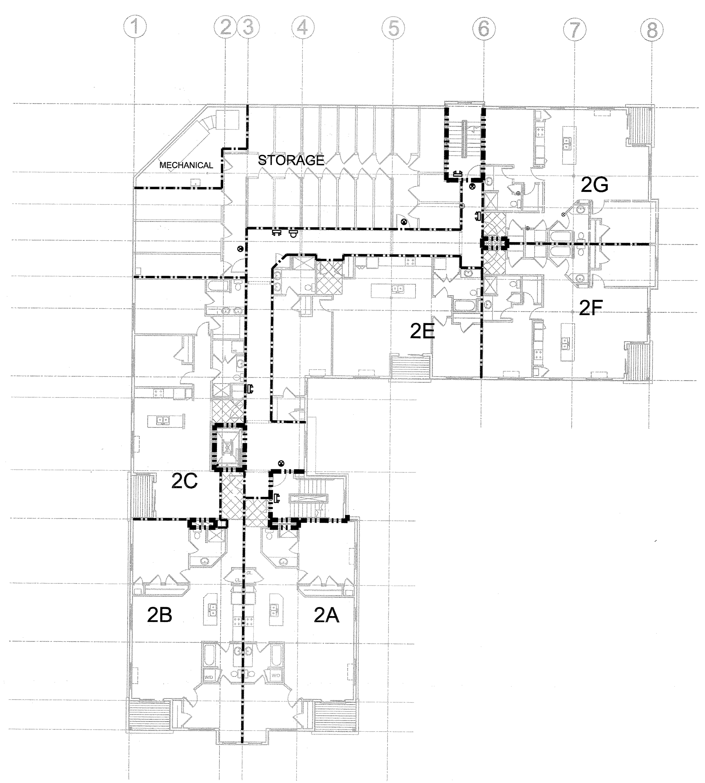
2 G1.2 SECOND FLOOR LIFE SAFETY PLAN 3/32" = 1'-0"
